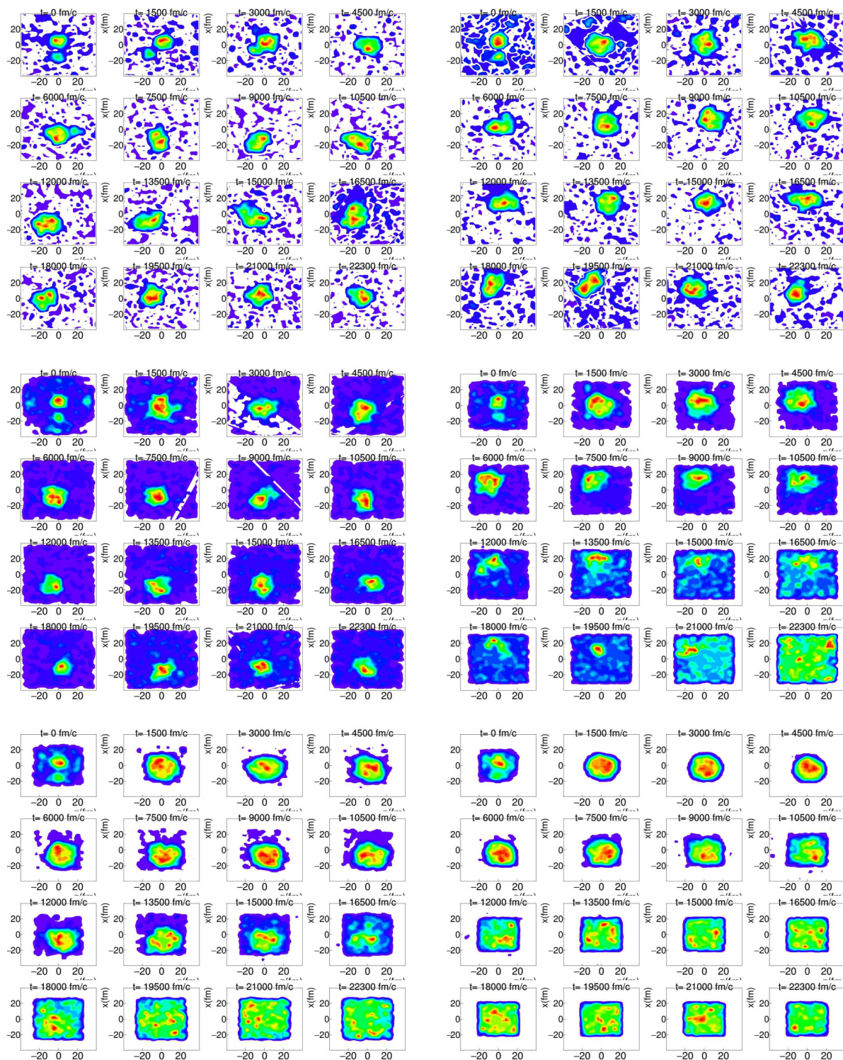
FIG. 2. Evolution of the system ^{140}\text{Ni} + ^{460}\text{U} in the nucleon bath with 10% proton concentration calculated using the CoMD code at beam energy 0.01 MeV/nucleon and Coulomb interaction cutoff at 10, 7, 5, 4, 3, and 2 fm (from top to bottom and left to right), corresponding to nucleon bath densities \rho_0/100 , \rho_0/50 , \rho_0/30 , \rho_0/17 , \rho_0/10 , and \rho_0/5 , respectively. Incompressibility is K_0 = 254 MeV and a soft density dependence of symmetry energy were used. The initial distance is 25 fm. On the time scale up to 25000 fm/c the resulting nucleus appears to dissolve in the nucleon bath with density above \rho_0/30 , even sooner with increasing density.
