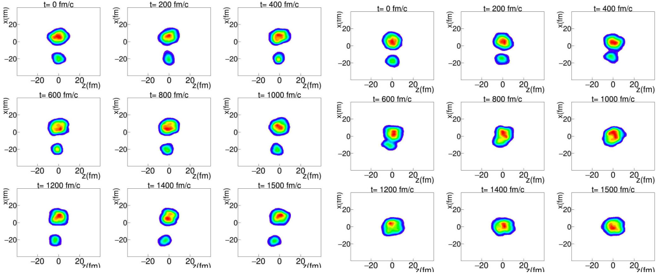
FIG. 1. Typical evolution of nucleonic density for central collision ^{140}\text{Ni} + ^{460}\text{U} calculated using the CoMD code at beam energy 1.25 MeV/nucleon (left panel) and 1.5 MeV/nucleon (right panel). A Coulomb interaction cutoff 2 fm, incompressibility K_0 = 254 MeV and a soft density dependence of symmetry energy were used. Scattering due to a “neutron wind” dominates at lower beam energy (left panel), while fusion dominates at higher beam energy (right panel).
