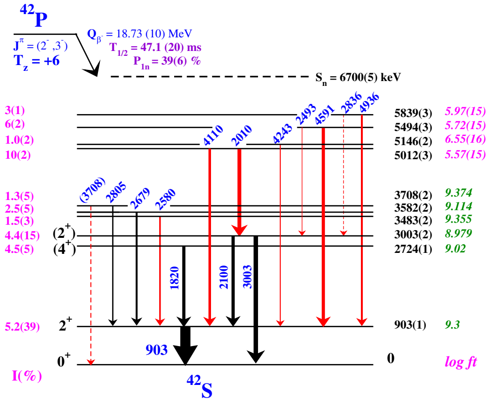
FIG. 4. Partial level scheme of ^{42}\text{S} following \beta decay of ^{42}\text{P} with a T_{1/2} = 47.1(20) \text{ ms} and Q_{\beta^-} = 18.73(10) \text{ MeV} . The transitions marked black were known before, whereas red indicates the new transitions. The absolute branching for each level was calculated using the measured yield in the gamma transition, total number of implants from the decay curve, and the \gamma detection. The width of the arrows are approximately proportional to the absolute intensity. The \log ft values were calculating using the \log ft calculator [31]. For levels above 5 MeV, they represent GT transitions while below indicate FF.
