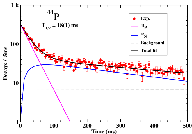
FIG. 8. The decay curve for ^{44}\text{P} and fitted in the same manner as ^{43}\text{P} .
