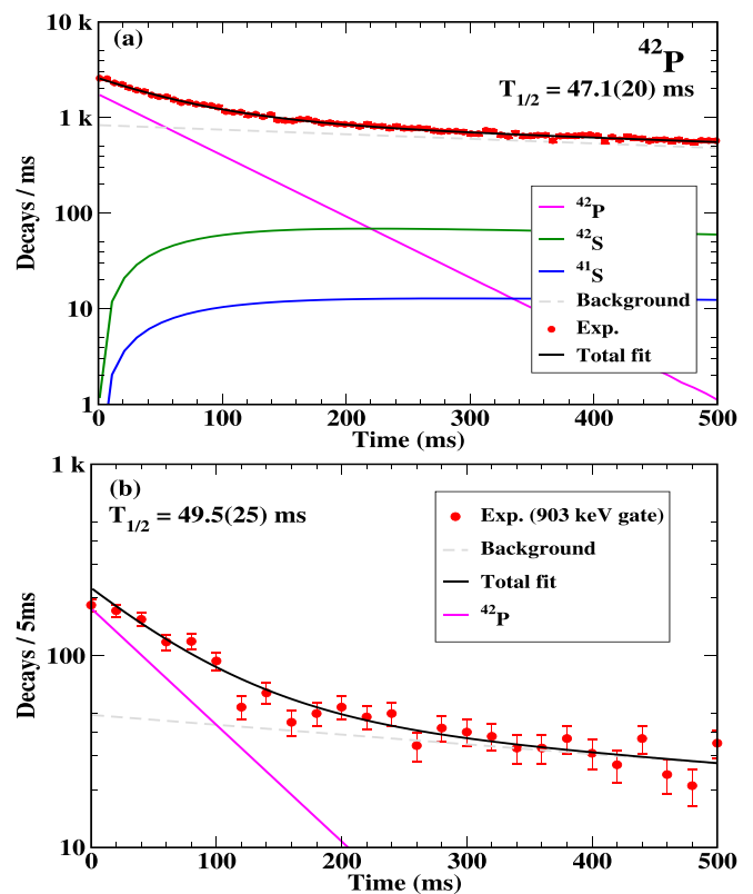
FIG. 1. (a) Decay curve derived for ^{42}\text{P} from \beta -correlated implants within a grid of nine pixels for 500 ms along with the fit used to extract half-life and the initial activity. The components of the fit are (i) exponential decay of parent, ^{42}\text{P} ; (ii) exponential growth and decay of daughter nuclei, ^{42}\text{S} ( \beta ) and ^{41}\text{S} ( \beta n ); and (iii) exponential background. Known half-lives were used for the daughter nuclides [31]. (b) Decay curve gated by the 903-keV transition which represents the 2^+ \rightarrow 0^+ transition in the daughter ^{42}\text{S} .
