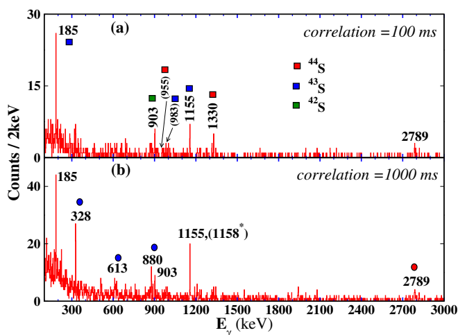
FIG. 9. \beta -delayed \gamma spectrum for ^{44}\text{P} (a) for a correlation window of 100 ms and (b) for 1000 ms. Transitions marked with red filled squares belong to \beta 0n daughter ^{44}\text{S} and red circles are the \beta 0n granddaughter ^{44}\text{Cl} . Blue filled squares are \beta 1n daughter ^{43}\text{S} and blue circles \beta 1n granddaughter ^{43}\text{Cl} , while green squares and circles are for the \beta 2n daughter and granddaughter ^{42}\text{S} and ^{42}\text{Cl} . The * in (b) indicates there is a doublet comprising the 1155- and 1158-keV transitions where the 1158-keV transition is from the long activity in either ^{44}\text{Ar} or ^{44}\text{K} .
