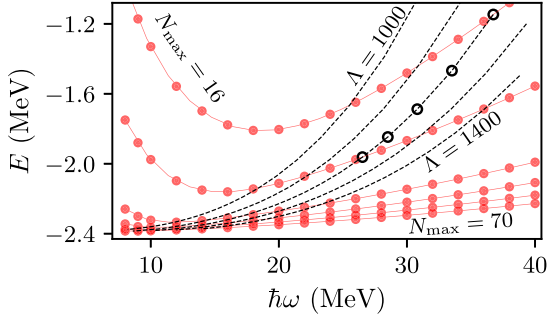
FIG. 3. The ground-state energy of {}^3_{\Lambda}\text{H} as a function of the HO frequency and Y-NCSM model space N_{\text{max}} . Results obtained with \text{NNLO}_{\text{sim}}(\Lambda_{\text{NV}} = 500 \text{ MeV}, T_{\text{Lab}}^{\text{max}} = 290 \text{ MeV}) at a subset of fixed N_{\text{max}} = \{16, 24, 40, 50, 60, 70\} are indicated by filled symbols connected by thin solid lines. Dashed lines indicate fixed UV scale \Lambda_{\text{UV}} = \{1000, 1100, 1200, 1300, 1400\} MeV. The benchmark IR extrapolation shown in Fig. 4 is performed with the GP-interpolated data indicated by open circles.
