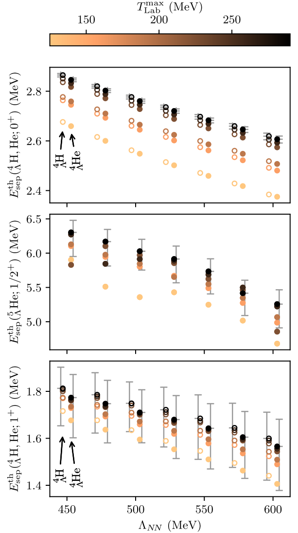
FIG. 7. Separation energies for {}^4_{\Lambda}\text{H} (open circles) and {}^4_{\Lambda}\text{He} (filled circles) ground and excited states for the family of \text{NNLO}_{\text{sim}} interactions. The data correspond to the medians from the Bayesian IR extrapolation. The 68% credible region from the IR extrapolation is indicated by the error bar for the seven T_{\text{Lab}}^{\text{max}} = 290 \text{ MeV} interactions in the \text{NNLO}_{\text{sim}} family.
