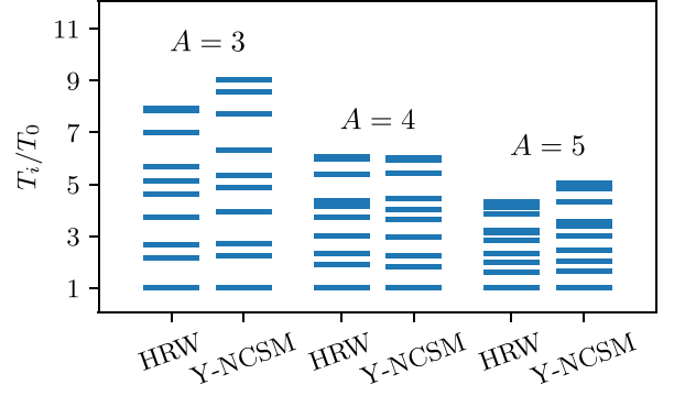
FIG. 1. Comparison of the discrete kinetic energy spectra for A = 3, 4, 5 hypernuclei in the Y-NCSM and in the corresponding D = 3(A - 1) dimensional hyper-radial well (HRW). In each case, the spectrum is plotted in units of the smallest eigenvalue.
