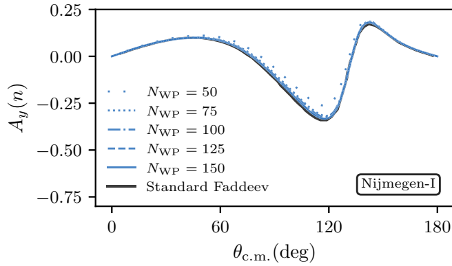
FIG. 2. The neutron analyzing power A_y(n) at E_{\text{Lab}} = 35 MeV vs c.m. scattering angle \theta_{\text{c.m.}} using the Nijmegen-I NN potential. The WPCD prediction approaches the standard Faddeev result [2] with an increasing number of wave packets N_{\text{WP}} and they overlap for N_{\text{WP}} \gtrsim 125 .
