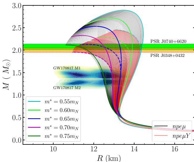
FIG. 2. Mass-radius relation corresponding to EoSs used in this work (see Fig. 1). Horizontal bands correspond to masses M = 2.072_{-0.066}^{+0.067} M_{\odot} of PSR J0740+6620 [11] (green band) and M = 2.01_{-0.04}^{+0.04} M_{\odot} of PSR J0348+0432 [8] (yellow band). The mass radius estimates of the two companion neutron stars in the merger event GW170817 [17] are shown by shaded area labeled with GW170817 M1 (M2) [52].
