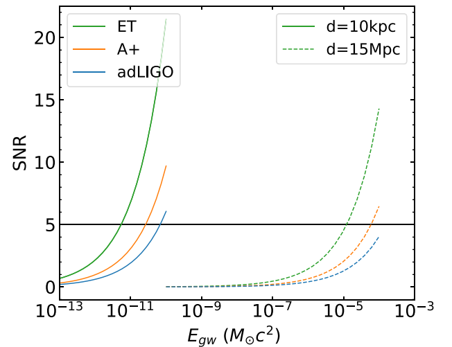
FIG. 12. Top panel: Gravitational wave strain corresponding to a maximum glitch energy observed in Vela pulsar (Crab pulsar) with distance to be 290 pc (2 kpc) are shown along with the sensitivity bands of different configurations. The waveforms are generated using the GW inference package Bilby [92]. Lower panel: Signal-to-noise ratio (SNR) for a source with f -mode frequency 1.70 kHz and damping time 0.25 s at different detector configurations as a function of E_{GW} for sources to be at 10 kpc (solid lines) or at 15 Mpc (dashed lines).
