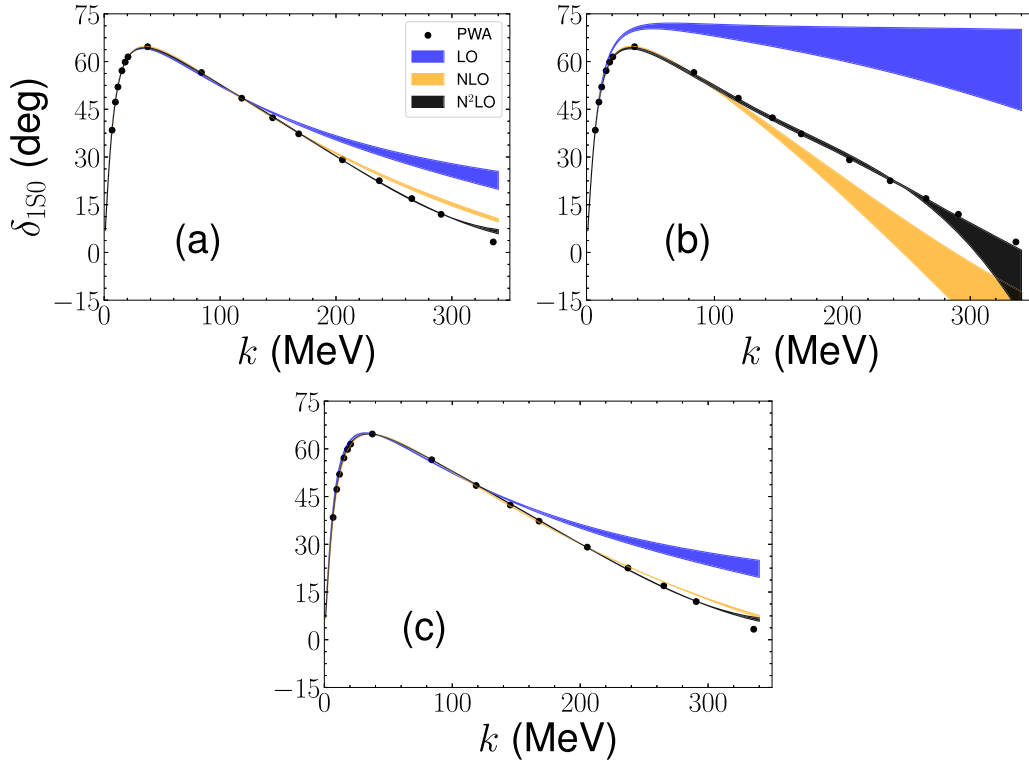
FIG. 2. The ^1S_0 phase shifts as a function of c.m. momentum k up to N^2 LO. The blue, orange and black bands represent LO, NLO, and N^2 LO respectively, and the bands show the variation with \Lambda from 600 to 2400 MeV. The potentials used in (a), (b), and (c) are momentum-dependent dibaryon potentials, MMW scheme and dynamic dibaryon potentials, respectively.
