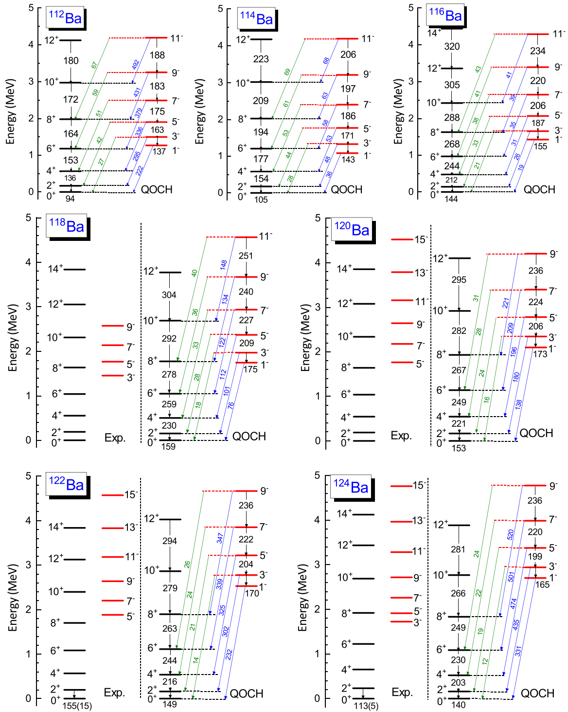
FIG. 18. The excitation spectrum, intraband B(E2) (W. u.) (in black), interband B(E1) ( \times 10^{-5} W. u.) (in blue) and B(E3) (W. u.) (in green) values of ^{112-124}\text{Ba} calculated with the QOCH based on DD-PC1 relativistic density functional, compared to experimental results.
