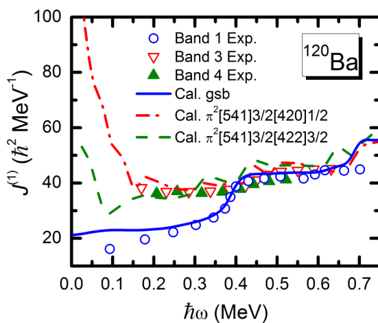
FIG. 12. Moment of inertia J^{(1)} for bands 1, 3, and 4 of ^{120}\text{Ba} calculated using the PNC-CSM model assuming reflection-asymmetric shapes with deformation parameters \epsilon_2 = 0.32 , \epsilon_2 = 0.003 .
