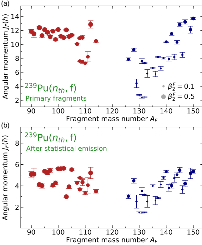
FIG. 1. Average angular momentum J_F of the heavy (blue) and light (red) fission fragments in ^{239}\text{Pu}(n_{th}, f) as a function of their mass number A_F . (a) Average AM of primary fission fragments calculated with microscopic theory. (b) Average AM of the fragments after the emission of neutrons and statistical photons was simulated with FREYA. In both panels, the area of the circles is proportional to the quadrupole deformation parameter \beta_2^F extracted for the fragments at scission. Note that the legend is illustrative and does not represent two discrete cases. The error bars in both panels represent the \pm 2\sigma_F^{\text{GP}} confidence intervals stemming from the Gaussian process interpolation for integer numbers of nucleons in FFs, where \sigma_F^{\text{GP}} = \sum_J \left| \frac{\partial J_F(J_F+1)}{\partial |a_J|^2} \sigma(|a_J|^2) \right| / (2J_F + 1) .
