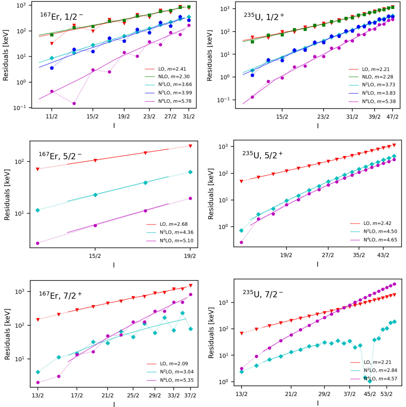
FIG. 9. Energy residuals for the 1/2^- , 5/2^- , and 7/2^+ rotational bands in ^{167}\text{Er} (left column) and for the 1/2^+ , 5/2^+ , and 7/2^- rotational bands in ^{235}\text{U} (right column) on a log-log scale. Experimental values are taken from the NNDC [26,28]. The red triangles, green squares, cyan diamonds, blue pentagons, and magenta circles are the residuals from the calculated energies at LO, NLO, \text{N}^2\text{LO} , \text{N}^3\text{LO} , and \text{N}^4\text{LO} , respectively. The dashed transparent lines are there to guide the eye. The solid lines show the trend of the calculated residuals after averaging out the signature staggering. The slope shown in the legend is the slope of the solid lines. For the 7/2^- rotational band in ^{235}\text{U} we see an accidental decrease in the residuals beyond I = 29/2 at \text{N}^2\text{LO} . Therefore, we do not include the points beyond I = 29/2 when calculating the slope.
