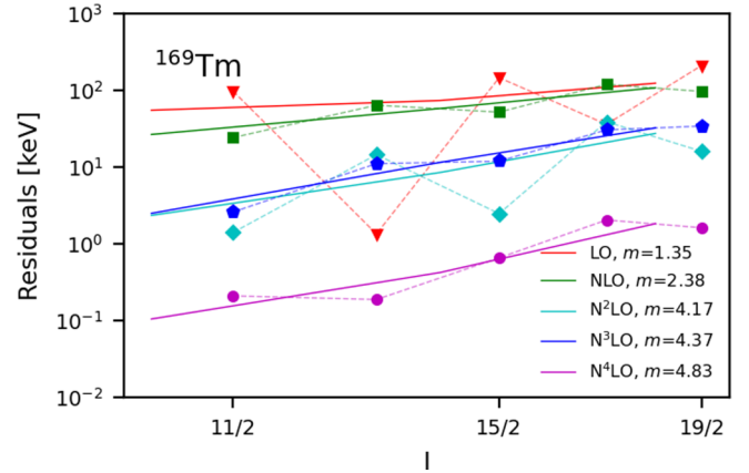
FIG. 13. Energy residuals for the 1/2^+ ground-state rotational band in ^{169}\text{Tm} on a log-log scale. The red triangles, green squares, cyan diamonds, blue pentagons and magenta circles are the residuals from the calculated energies at LO, NLO, N^2\text{LO} , N^3\text{LO} , and N^4\text{LO} , respectively. The dashed transparent lines are there to guide the eye. The solid lines show the trend of the calculated residuals after averaging out the signature staggering. The slope shown in the legend is the slope of the solid lines.
