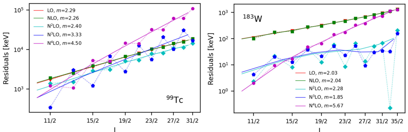
FIG. 11. Energy residuals for states in the 1/2^- excited-state rotational band in ^{99}\text{Tc} (left panel) and in the 1/2^- ground-state rotational band in ^{183}\text{W} (right panel) on a log-log scale. The red triangles, green squares, cyan diamonds, blue pentagons and magenta circles are the residuals from the calculated energies at LO, NLO, \text{N}^2\text{LO} , \text{N}^3\text{LO} , and \text{N}^4\text{LO} , respectively. The dashed transparent lines are there to guide the eye. The solid lines show the trend of the calculated residuals after averaging out the signature staggering. The slope shown in the legend is the slope of the solid lines.
