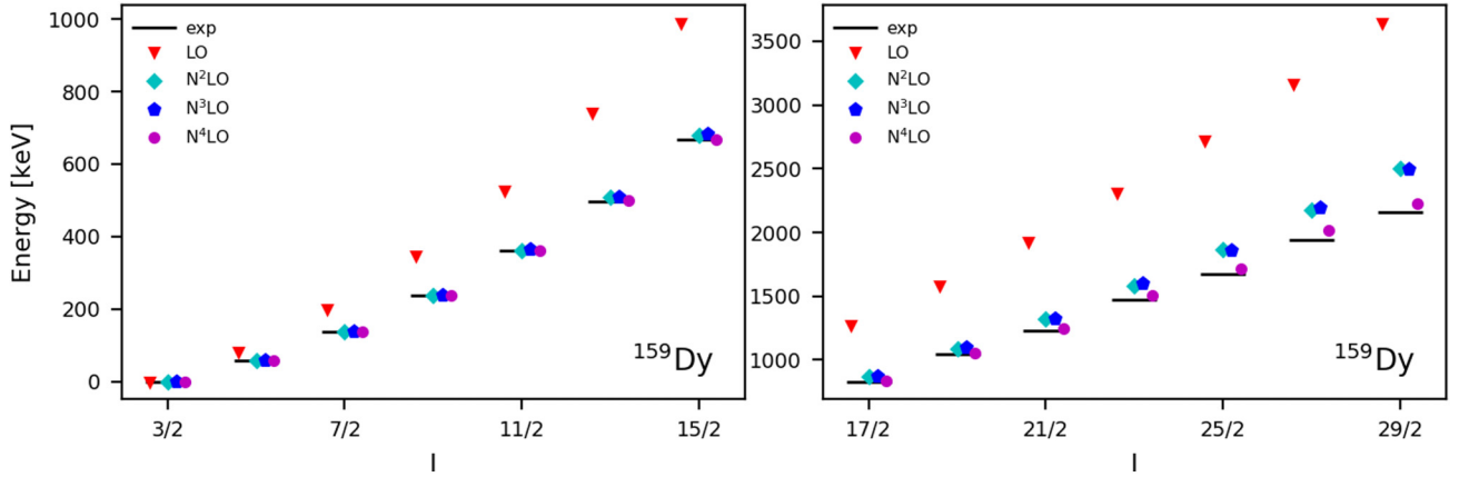
FIG. 7. Calculated energies for states in the 3/2^- ground-state rotational band in ^{159}\text{Dy} . The black lines show the experimental values taken from the NNDC [29]. The red triangles, cyan diamonds, blue pentagons and magenta circles are the calculated energies at LO, \text{N}^2\text{LO} , \text{N}^3\text{LO} , and \text{N}^4\text{LO} , respectively. The right panel is a continuation of the left panel with a different scale on the y axis.
