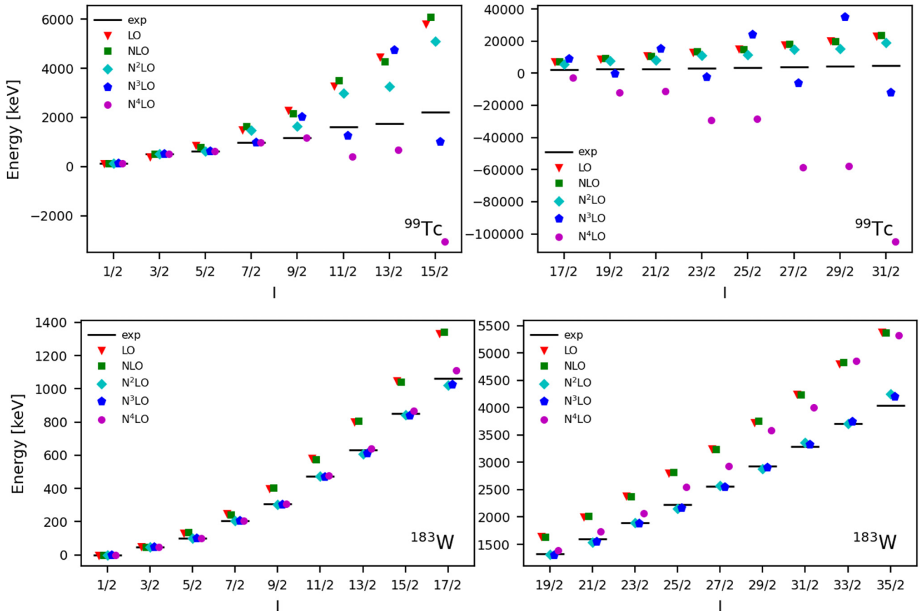
FIG. 10. Calculated energy for states in the 1/2^- excited-state rotational band in ^{99}\text{Tc} (top panels) and in the 1/2^- ground-state rotational band in ^{183}\text{W} (bottom panels). The black line shows the experimental values taken from the NNDC [30,31]. The red triangles, green squares, cyan diamonds, blue pentagons and magenta circles are the calculated energies at LO, NLO, \text{N}^2\text{LO} , \text{N}^3\text{LO} , and \text{N}^4\text{LO} , respectively. The right panel is a continuation of the left panel with a different scale for the y axis.
