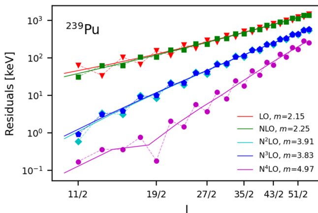
FIG. 6. Energy residuals for the 1/2^+ ground-state rotational band in ^{239}\text{Pu} on a log-log scale. The red triangles, green squares, cyan diamonds, blue pentagons, and magenta circles are the residuals from the calculated energies at LO, NLO, \text{N}^2\text{LO} , \text{N}^3\text{LO} , and \text{N}^4\text{LO} , respectively. The dashed transparent lines are there to guide the eye. The solid lines show the trend of the calculated residuals after averaging out the signature staggering. The slope shown in the legend is the slope of the solid lines.
