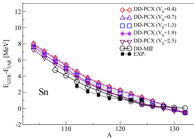
FIG. 6. The PN-RQRPA excitation energy for GT - direct spin-flip transitions for 104–132 Sn, for the range of values of the isoscalar proton-neutron pairing interaction strength parameter V_0 . Calculations are based on the density-dependent point coupling interaction DD-PCX and the results from the previous study based on the DD-ME2 interaction [6] and the experimental data from Ref. [4] are shown for comparison.
