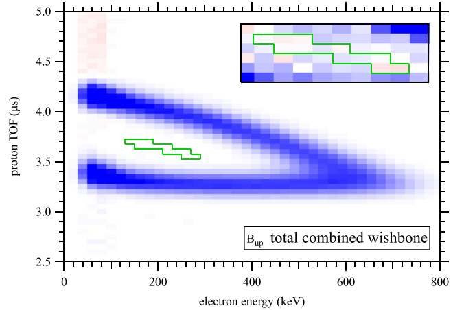
FIG. 23. A combined background-subtracted wishbone plot with all B_{\text{up}} data. The event total in the region outlined in green was used to test for the presence of a low-energy tail in the detected electron response function due to electron scattering. The inset shows the same green-outlined region with an expanded color scale. Blue points are positive counts, red points are negative due to the background subtraction.
