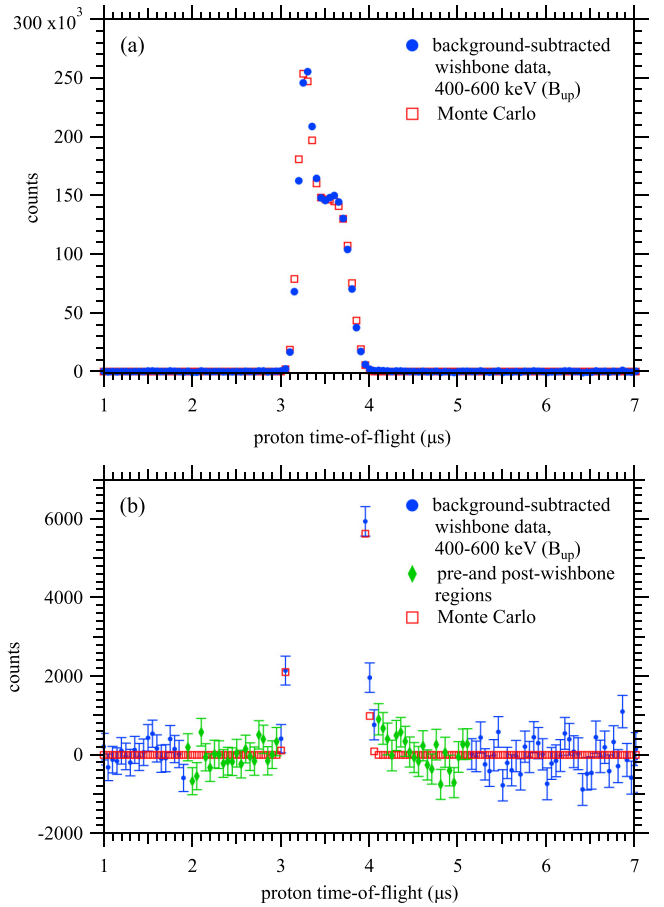
FIG. 25. (a) The total B_{\text{up}} wishbone proton TOF spectrum summed from 400 to 600 keV compared to the equivalent Monte Carlo proton TOF spectrum. (b) The same plot with an expanded vertical scale and statistical error bars. The 1 \mu\text{s} wide regions pre- and post-wishbone used to estimate the proton scattering tail are shown in green.
