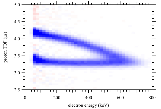
FIG. 17. A background-subtracted wishbone plot (data from Fig. 13). Blue points are positive and red are negative.
