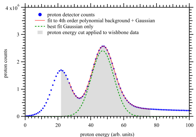
FIG. 24. A typical proton energy spectrum (blue) fit to a fourth-order polynomial background function plus a Gaussian (red). The resulting Gaussian alone is shown in green. The soft energy threshold of the PIXIE-16 takes effect below channel 27. The slight loss of protons below threshold has a negligible effect on the wishbone asymmetry.
