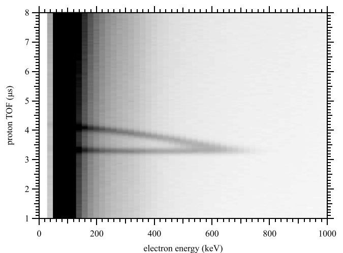
FIG. 13. A typical raw wishbone obtained from approximately 100 hours of reduced data, using the proton energy cut shown in Fig. 12.
