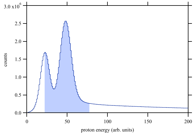
FIG. 12. A typical proton energy singles spectrum. The peak on the right is protons. The noise/background forms a peak on the left due to the soft energy threshold of the PIXIE. The shaded region is the applied proton energy window.
