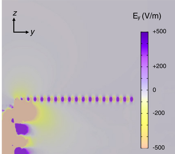
FIG. 21. A COMSOL finite element map of the transverse electric field inside the NG-C electrostatic mirror, in the region near the upper wire grid through which the protons pass.
