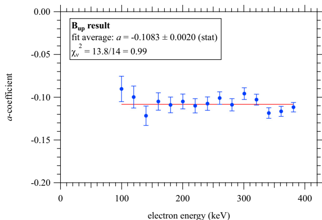
FIG. 27. The corrected B_{\text{up}} wishbone asymmetry (see Fig. 20), divided by the geometric function f_a(E) (see Fig. 4), giving the measured a coefficient for each beta-energy slice. These were fit to a constant to produce the a -coefficient result for the B_{\text{up}} data. Error bars are statistical.
