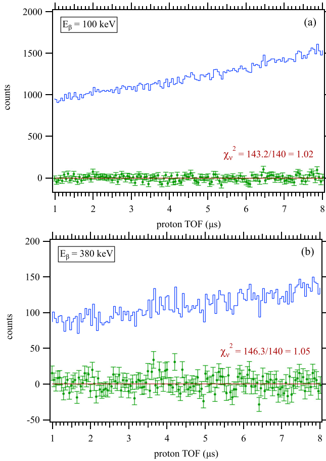
FIG. 16. The 20-keV wide wishbone slices centered at (a) 100 and (b) 380 keV for a data series where the polarity of the electrostatic mirror was reversed, so neutron-decay protons could not be detected. The upper curve (blue) is the raw wishbone and the lower curve (green) is after subtracting background and fitting to a horizontal line. Error bars are statistical.
