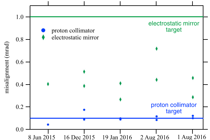
FIG. 11. A summary of optical insert alignment checks made over the course of the run. Multiple points are independent measurements made by two people.
