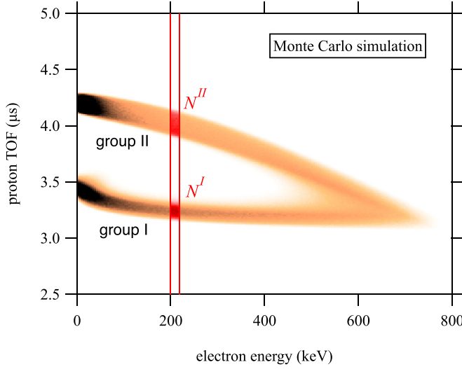
FIG. 3. A Monte Carlo simulation of aCORN data, proton TOF vs. beta energy for coincidence events. The fast proton branch (group I) is associated with neutron decays where the antineutrino momentum was in region I in Fig. 2. The slow proton branch (group II) is associated with decays where the antineutrino momentum was in region II. The sums N^I and N^{II} are used to compute the wishbone asymmetry for each beta-energy slice.
