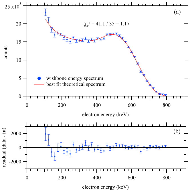
FIG. 18. (a) The wishbone energy spectrum, i.e., the background subtracted wishbone (Fig. 17) summed over proton TOF and the best fit theoretical spectrum. (b) Fit residuals (data minus fit). Error bars are statistical.
