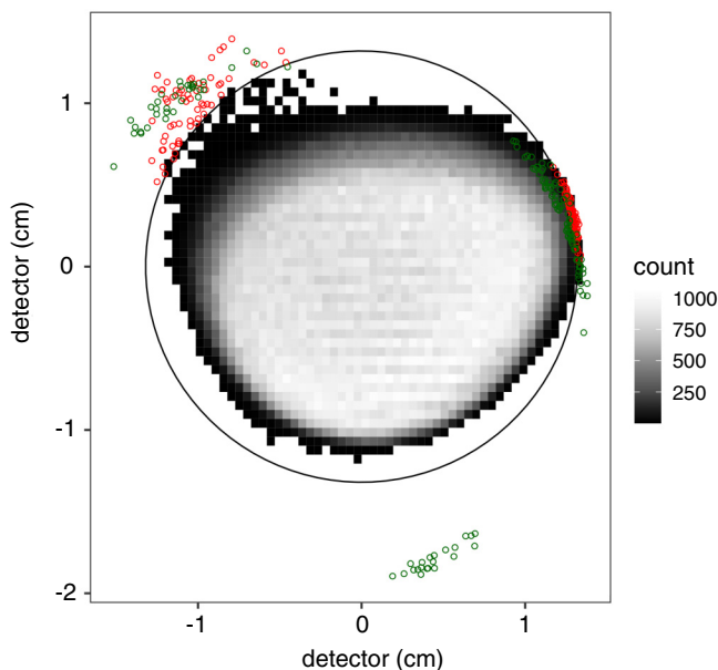
FIG. 26. Results from a proton focusing simulation tracking 1 million neutron-decay protons from the proton collimator to the detector. Green and red circles are protons striking the focusing ring and detector inactive region, respectively. The thin black circle indicates the active region of the surface barrier detector.
