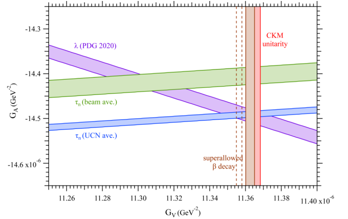
FIG. 1. A summary of experimental constraints on the nucleon weak coupling constants G_A and G_V . The purple band is the PDG 2020 [6] recommended value for \lambda from neutron-decay parameters A and a , including a scale factor of \sqrt{\chi_p^2} = 2.6 to account for poor agreement among experiments. The green (no scale factor) and blue (scale factor \sqrt{\chi_p^2} = 1.5 ) bands are derived from the neutron lifetime averages for the beam and UCN storage experiments. The brown vertical band shows G_V from superallowed beta decay [10] and the dashed lines indicate the shift due to the calculation of \Delta_R by Seng et al. [11]. The red vertical band shows the CKM matrix unitarity condition using the PDG recommended value of V_{us} [6].
