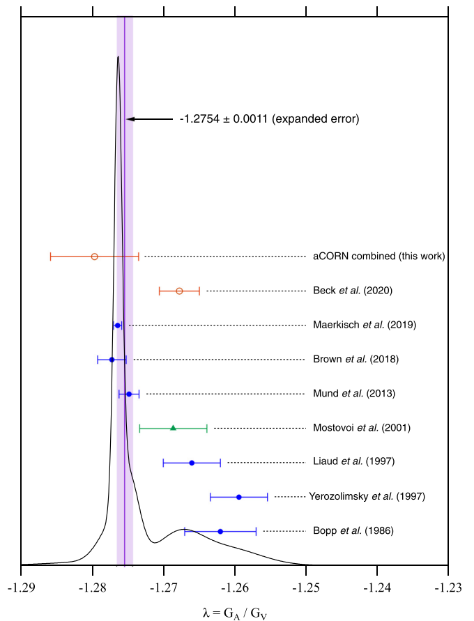
FIG. 30. An ideogram of precision determinations of the neutron-decay ratio of axial vector to vector coupling ( \lambda ) using the beta asymmetry ( A coefficient, blue circles), the electron-antineutrino correlation ( a coefficient, red open circles), and the A/B ratio (green triangle). The distribution features two groups of experimental results and the overall agreement is poor. The weighted average is indicated with the uncertainty expanded by a factor of 2.32.
