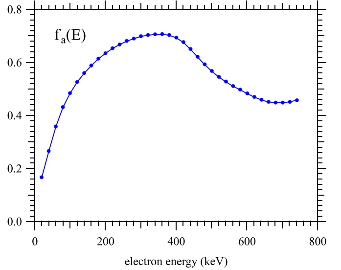
FIG. 4. The dimensionless geometric function f_a(E) , computed numerically from the aCORN geometry and a 36.4-mT uniform magnetic field [see Eqs. (8) and (9)].
