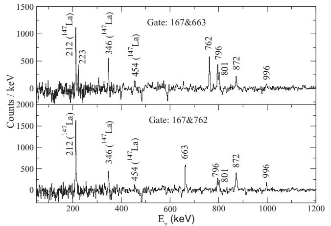
FIG. 1. Double-gated \gamma\gamma\gamma -coincidence spectra with one gate set on the strong 167 keV ^{147}\text{La} transition and the other gate set on one of the ^{87}\text{Br} candidate transitions.
