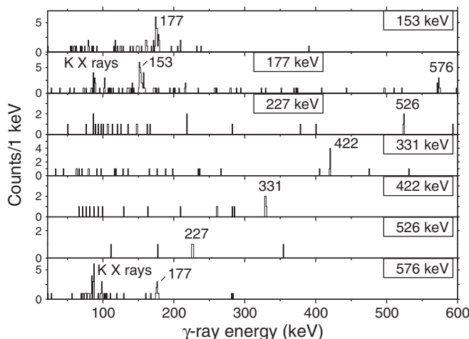
FIG. 7. \gamma\gamma -coincidence spectra, following the \alpha decay of ^{221}\text{Th} . The energy of the \gamma -ray gate is indicated on each panel.
