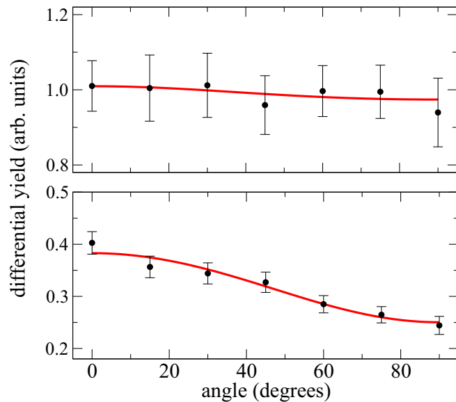
FIG. 4. Angular distributions of \gamma rays at E_\alpha = 4.822 MeV ( E_{c.m.} = 4.132 MeV, E_x = 14.117 MeV) for the ^{24}\text{Mg}(\alpha, p_1)^{27}\text{Al} and ^{24}\text{Mg}(\alpha, p_2)^{27}\text{Al} reactions are shown in the top and bottom plots, respectively. The solid red line shows the Legendre polynomial fit.
