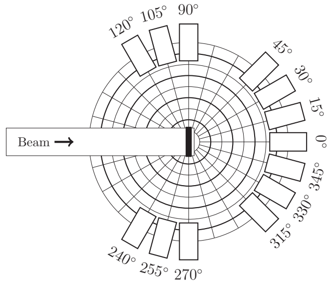
FIG. 1. A schematic of the experimental setup. The detectors are of type \text{LaBr}_3 from the HAGRiD array, which were used to measure angular distributions of secondary \gamma rays from the ^{24}\text{Mg}(\alpha, p_{1,2}\gamma)^{27}\text{Al} reaction. The water-cooled target is indicated by the black rectangle in the center of the HAGRiD array.
