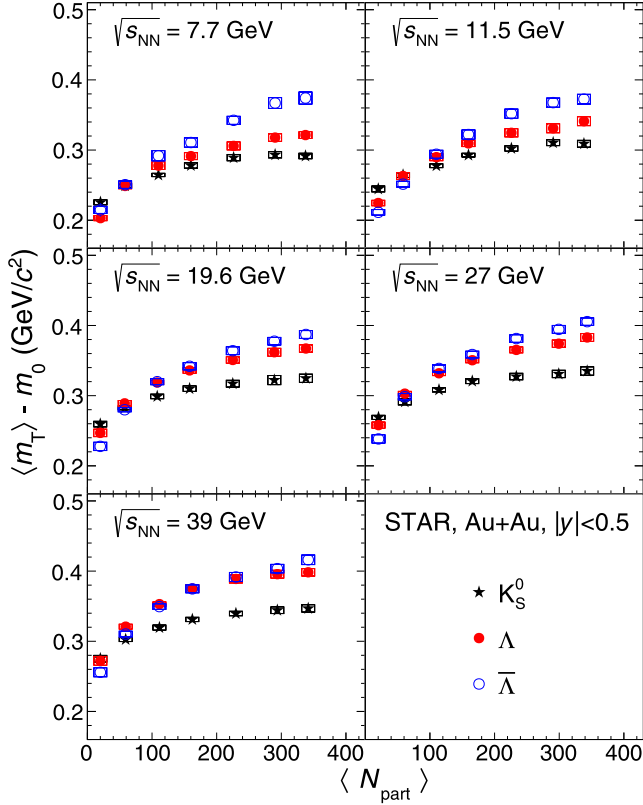
FIG. 13. The averaged transverse mass, \langle m_T \rangle - m_0 , at midrapidity ( |y| < 0.5 ) for K_S^0 , \Lambda , and \bar{\Lambda} as a function of \langle N_{\text{part}} \rangle for Au + Au collisions at \sqrt{s_{NN}} = 7.7 –39 GeV. The box on each data point denotes the systematic error.
