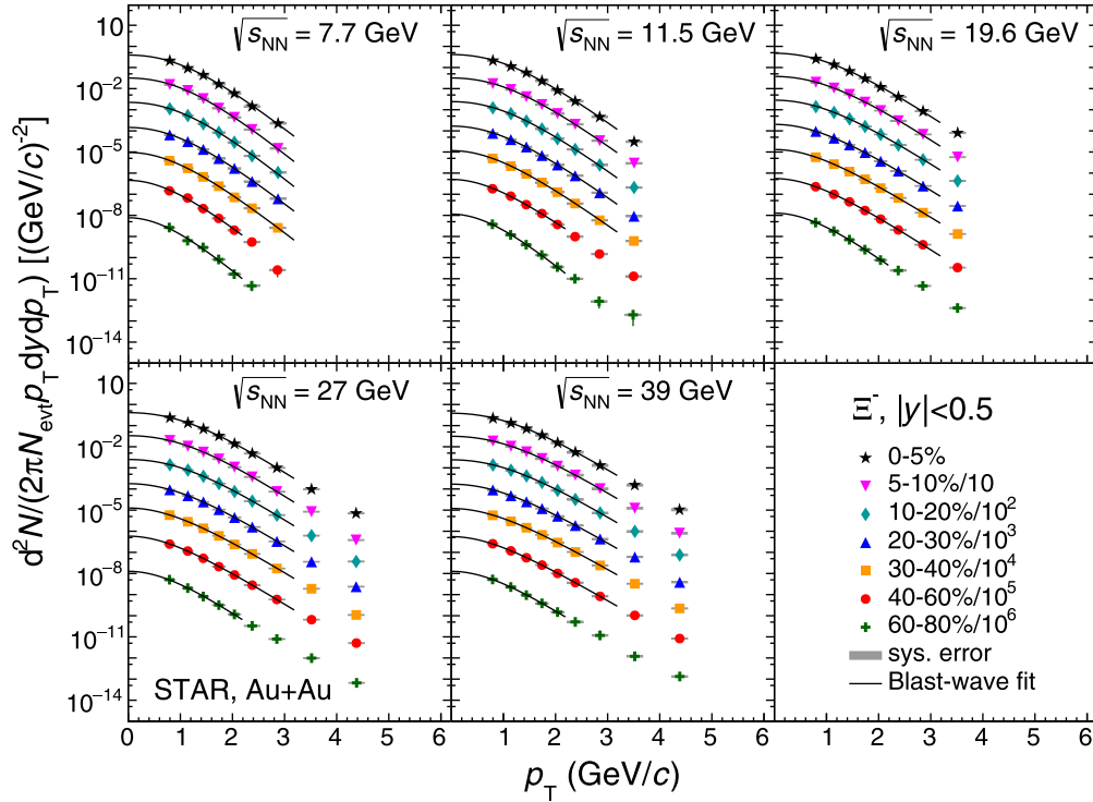
FIG. 8. The transverse-momentum spectra of \Xi^- at midrapidity ( |y| < 0.5 ) from Au + Au collisions at different centralities and energies ( \sqrt{s_{NN}} = 7.7\text{--}39 GeV). The data points are scaled by factors of 10 from central to peripheral collisions for clarity. The vertical gray bands represent the systematic errors, which are small hence the bands look like horizontal bars. The blast-wave model fit results are shown in the fit range and the low- p_T extrapolation range as solid lines for all centrality bins.
