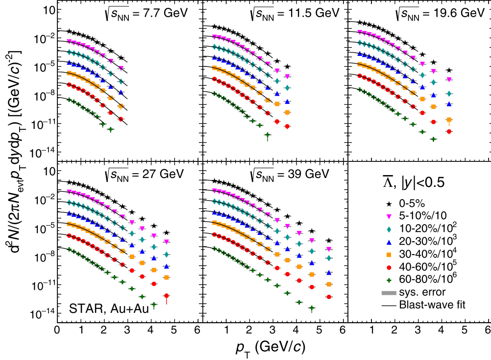
FIG. 7. The transverse-momentum spectra of \bar{\Lambda} at midrapidity ( |y| < 0.5 ) from Au + Au collisions at different centralities and energies ( \sqrt{s_{NN}} = 7.7\text{--}39 GeV). The spectra are corrected for the feed-down of \bar{\Xi}^+ , \bar{\Xi}^0 , and \bar{\Omega}^+ decays. The data points are scaled by factors of 10 from central to peripheral collisions for clarity. The vertical gray bands represent the systematic errors, which are small hence the bands look like horizontal bars. The blast-wave model fit results are shown in the fit range and the low- p_T extrapolation range as solid lines for all centrality bins.
