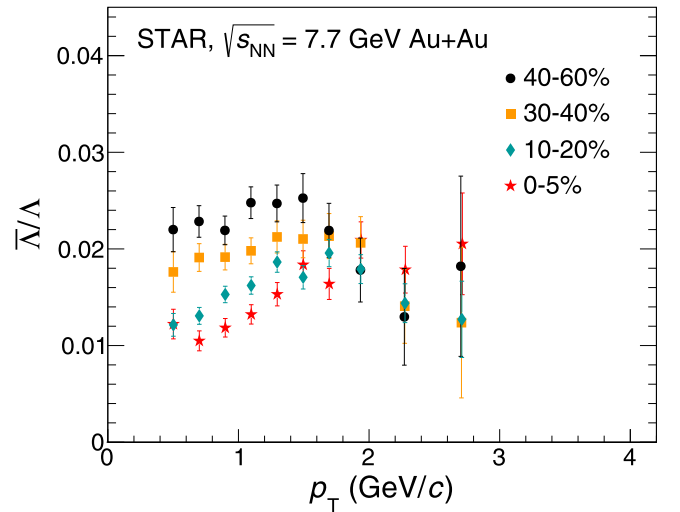
FIG. 21. \bar{\Lambda}/\Lambda ratio as a function of p_T from different centralities of Au + Au collisions at \sqrt{s_{NN}} = 7.7 GeV. The errors are statistical only.
