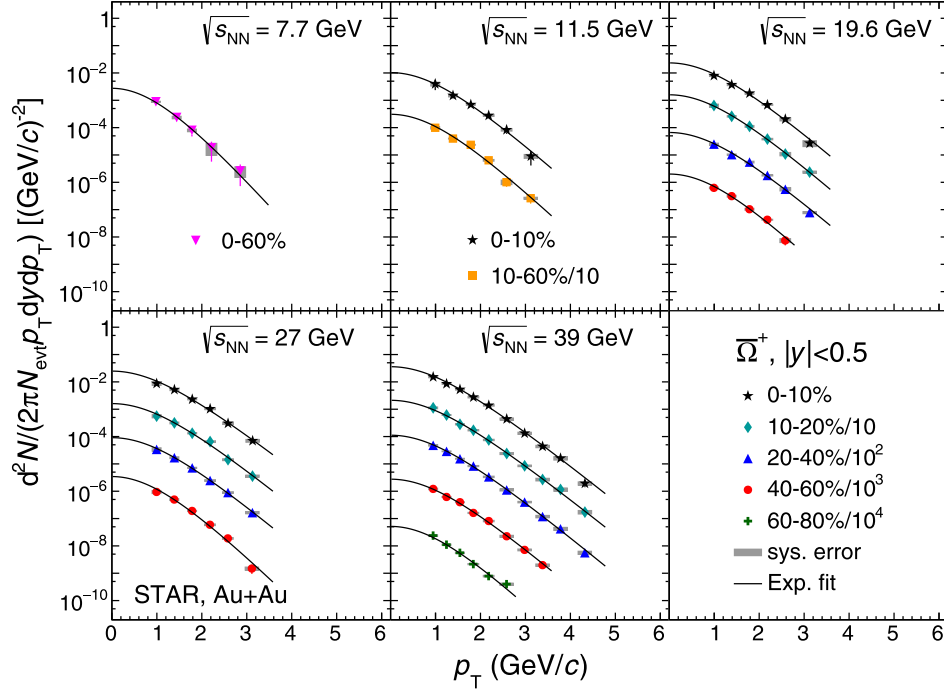
FIG. 11. The transverse-momentum spectra of \bar{\Omega}^+ at midrapidity ( |y| < 0.5 ) from Au + Au collisions at different centralities and energies ( \sqrt{s_{NN}} = 7.7\text{--}39 GeV). The data points are scaled by factors of 10 from central to peripheral collisions for clarity. The vertical gray bands represent the systematic errors, which are small hence the bands look like horizontal bars. The exponential function fit results are shown in the fit range and the low- p_T extrapolation range as solid lines for all centrality bins.
