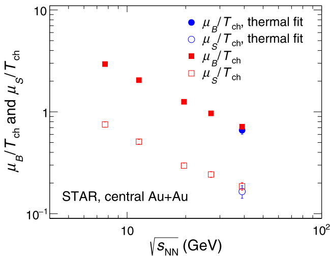
FIG. 26. The \mu_B/T_{\text{ch}} and \mu_S/T_{\text{ch}} parameters (red symbols) in central Au + Au collisions at \sqrt{s_{\text{NN}}} = 7.7\text{--}39 GeV obtained from the fits shown in Fig. 25. The blue symbols are the corresponding results from the thermal model fit to the yields of \pi , K, p , \Lambda , \Xi , K_S^0 , and \Omega at \sqrt{s_{\text{NN}}} = 39 GeV [7].
