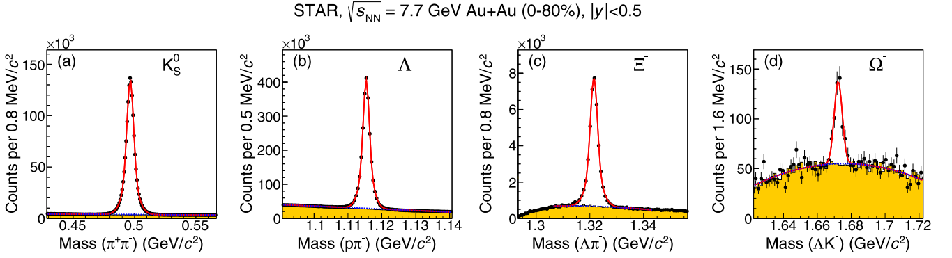
FIG. 1. K_S^0 , \Lambda , \Xi^- , and \Omega^- invariant mass distributions in Au + Au collisions at \sqrt{s_{NN}} = 7.7 GeV. The red solid lines represent the function fit results (double Gaussian plus polynomial for K_S^0 , \Lambda , and \Xi^- ; single Gaussian plus polynomial for \Omega^- ), and the blue dashed lines are the fitted background contributions. The orange area shows the corresponding rotational background distribution.
