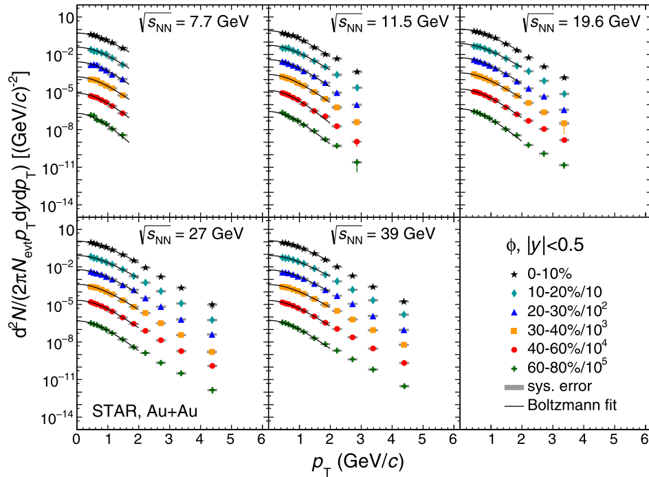
FIG. 12. The transverse-momentum spectra of \phi at midrapidity ( |y| < 0.5 ) from Au + Au collisions at different centralities and energies ( \sqrt{s_{NN}} = 7.7\text{--}39 GeV). The data points are scaled by factors of 10 from central to peripheral collisions for clarity. The vertical gray bands represent the systematic errors, which are small hence the bands look like horizontal bars. The Boltzmann function fit results are shown in the fit range and the low- p_T extrapolation range as solid lines for all centrality bins.
