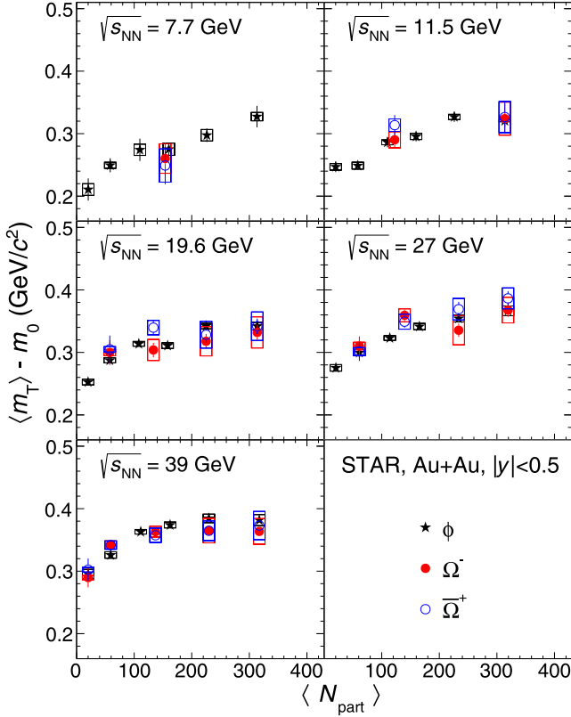
FIG. 15. The averaged transverse mass, \langle m_T \rangle - m_0 , at midrapidity ( |y| < 0.5 ) for \phi , \Omega , and \bar{\Omega} as a function of \langle N_{\text{part}} \rangle for Au + Au collisions at \sqrt{s_{NN}} = 7.7 –39 GeV. The box on each data point denotes the systematic error.
