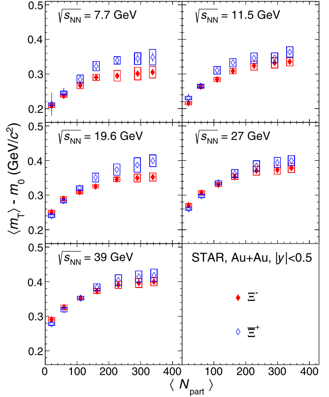
FIG. 14. The averaged transverse mass, \langle m_T \rangle - m_0 , at midrapidity ( |y| < 0.5 ) for \Xi^- and \bar{\Xi}^+ as a function of \langle N_{\text{part}} \rangle for Au + Au collisions at \sqrt{s_{NN}} = 7.7 –39 GeV. The box on each data point denotes the systematic error.
