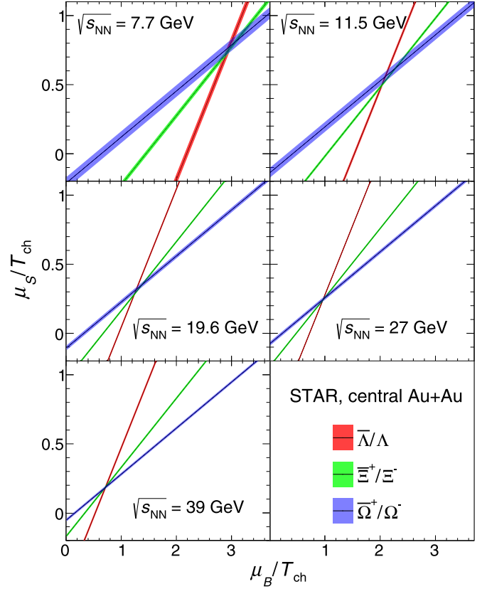
FIG. 24. Testing result of the thermal model in \mu_B/T_{ch} and \mu_S/T_{ch} parameter space with three strange antibaryon-to-baryon ratios in central Au + Au collisions at \sqrt{s_{NN}} = 7.7 –39 GeV. Errors are propagated from the corresponding \bar{B}/B ratios, whose errors are the quadratic sum of statistical and systematic errors.
