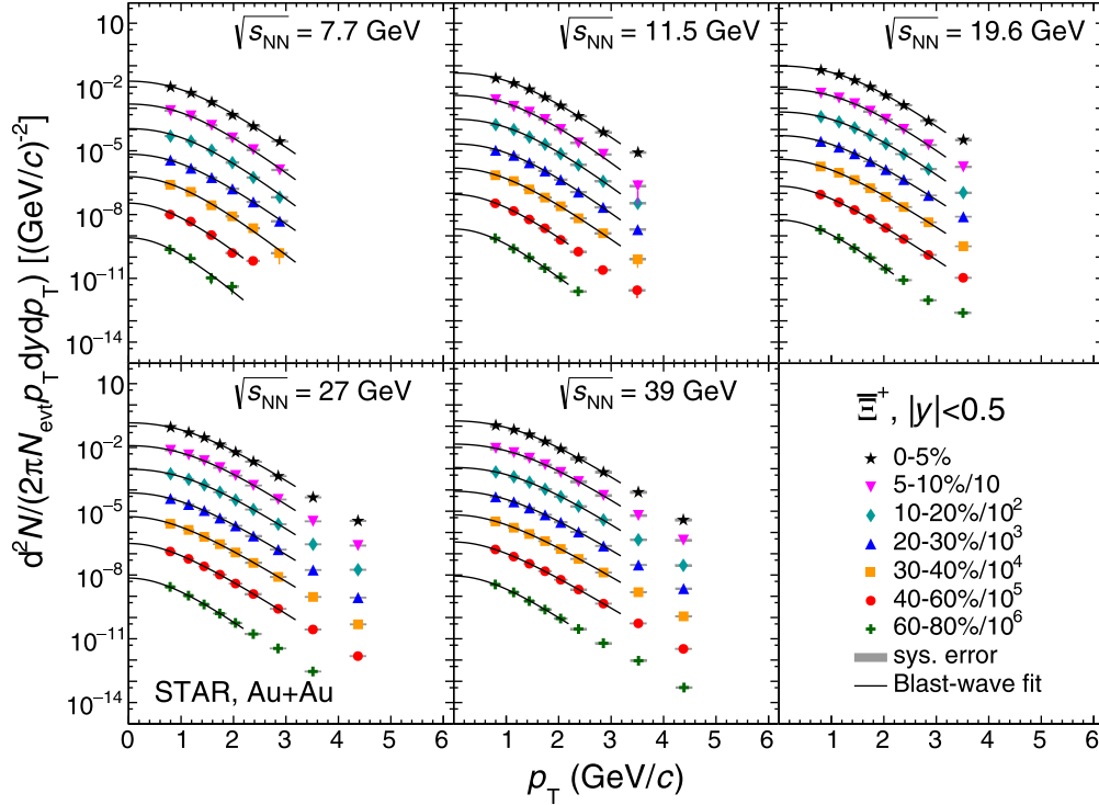
FIG. 9. The transverse-momentum spectra of \Xi^+ at midrapidity ( |y| < 0.5 ) from Au + Au collisions at different centralities and energies ( \sqrt{s_{NN}} = 7.7\text{--}39 GeV). The data points are scaled by factors of 10 from central to peripheral collisions for clarity. The vertical gray bands represent the systematic errors, which are small hence the bands look like horizontal bars. The blast-wave model fit results are shown in the fit range and the low- p_T extrapolation range as solid lines for all centrality bins.
