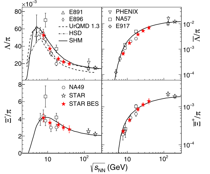
FIG. 27. Energy dependence of \Lambda , \bar{\Lambda} , \Xi^- , and \bar{\Xi}^+ to pions [ 1.5(\pi^+ + \pi^-) ] ratios at midrapidity in central Au + Au collisions from STAR Beam Energy Scan (solid symbols). The STAR BES midrapidity pion yields are taken from [7]. Errors are the quadratic sum of statistical and systematic errors. Also shown are existing AGS [14,15,17,18,78], NA49 [20,23,24,79], PHENIX [38,80], and STAR [29,31,32,37,81,82] data as open symbols, as well as calculations from hadronic transport models (UrQMD 1.3 and HSD) [83–86] and a statistical hadron gas model (SHM) [44] as dashed or solid lines. The E896, PHENIX, and NA57 8.7 GeV \bar{\Xi}^+/\pi data points are slightly shifted to the right for clarity.
