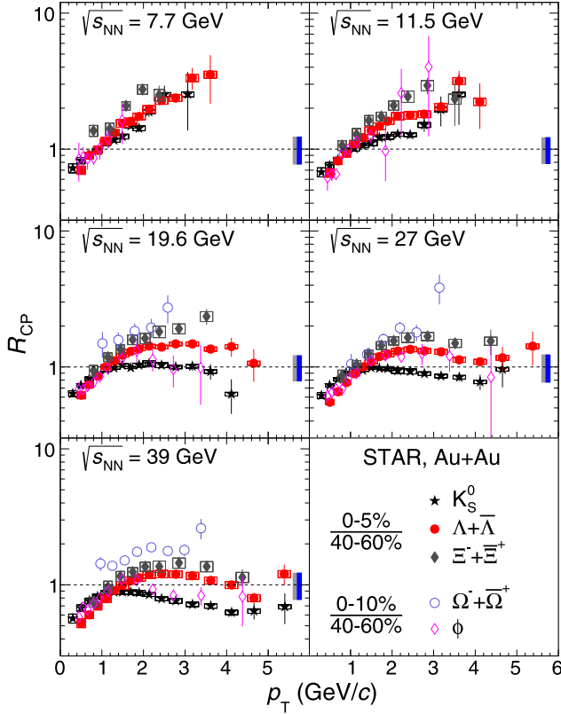
FIG. 28. K_S^0 , \Lambda + \bar{\Lambda} , and \Xi^- + \Xi^+ R_{CP}(0-5\%)/(40-60\%) , \phi and \Omega^- + \Omega^+ R_{CP}(0-10\%)/(40-60\%) , at midrapidity ( |y| < 0.5 ) in Au + Au collisions at \sqrt{s_{NN}} = 7.7-39 GeV. The vertical bars denote the statistical errors. The box on each data point of K_S^0 , \Lambda , and \Xi denotes the systematic error. There are only statistical errors for \Omega and \phi . For \sqrt{s_{NN}} \leq 19.6 GeV, the \Lambda + \bar{\Lambda} R_{CP} excludes the minor contribution from \bar{\Lambda} . The gray and blue bands on the right side of each panel represent the normalization errors from N_{coll} for R_{CP}(0-5\%)/(40-60\%) and R_{CP}(0-10\%)/(40-60\%) , respectively.
