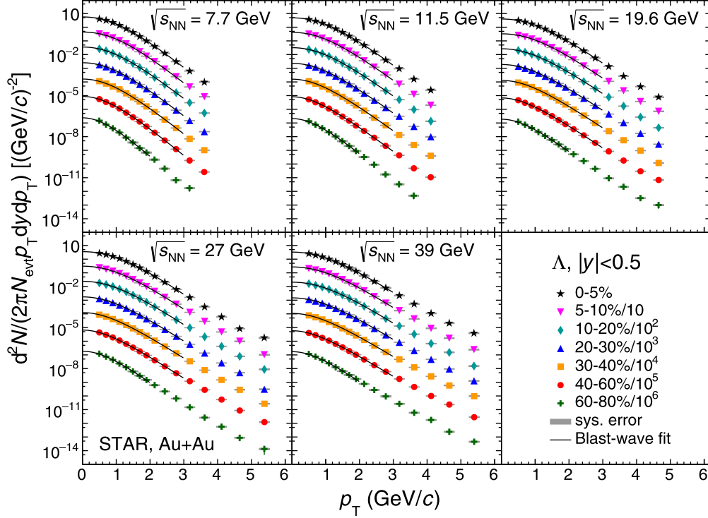
FIG. 6. The transverse-momentum spectra of \Lambda at midrapidity ( |y| < 0.5 ) from Au + Au collisions at different centralities and energies ( \sqrt{s_{NN}} = 7.7\text{--}39 GeV). The spectra are corrected for the feed-down of \Xi^- and \Xi^0 decays. The data points are scaled by factors of 10 from central to peripheral collisions for clarity. The vertical gray bands represent the systematic errors, which are small hence the bands look like horizontal bars. The blast-wave model fit results are shown in the fit range and the low- p_T extrapolation range as solid lines for all centrality bins.
