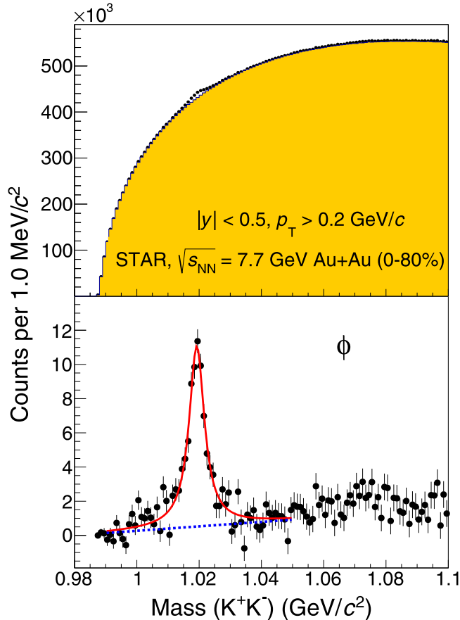
FIG. 2. \phi invariant mass distributions in Au + Au collisions at \sqrt{s_{NN}} = 7.7 GeV. The upper panel shows the unlike-charge invariant mass distribution (full points) and the mixed-event background (orange area). The lower panel shows the invariant mass distribution after subtracting the background. The red solid line represents the function fit result (Breit-Wigner plus polynomial), and the blue dashed line is the fitted residual background contributions.
