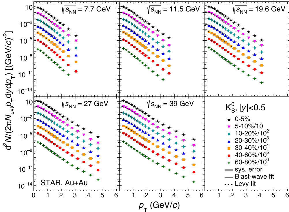
FIG. 5. The transverse-momentum spectra of K_S^0 at midrapidity ( |y| < 0.5 ) from Au + Au collisions at different centralities and energies ( \sqrt{s_{NN}} = 7.7 – 39 GeV). The data points are scaled by factors of 10 from central to peripheral collisions for clarity. The vertical gray bands represent the systematic errors, which are small hence the bands look like horizontal bars. The blast-wave model (or Levy function) fit results are shown in the fit range and the low- p_T extrapolation range as solid (dashed) lines for the centrality bins within 0–30% (30–80%).
