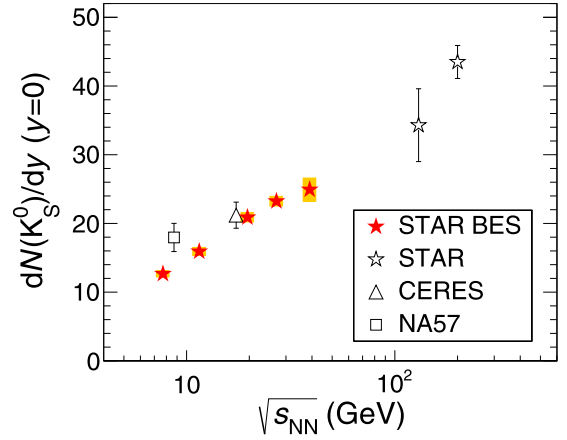
FIG. 18. The K_S^0 integrated yield, dN/dy , at midrapidity ( |y| < 0.5 ) as a function of collision energy from 0–5% central Au + Au collisions at \sqrt{s_{NN}} = 7.7\text{--}39 GeV. The orange shaded bands on the STAR BES data points represent the systematic errors. Also shown are the previous midrapidity results from 0–5% central Au + Au collisions at \sqrt{s_{NN}} = 130 and 200 GeV ( |y| < 0.5 ) from STAR [30,37], from 0–5% central Pb + Pb collisions at \sqrt{s_{NN}} = 8.7 GeV ( |y| < 0.5 ) from NA57 [26,27], and from 0–7% central Pb + Au collisions at \sqrt{s_{NN}} = 17.3 GeV from CERES [28]. CERES midrapidity data are the extrapolated values based on the measurements at backward rapidity.
