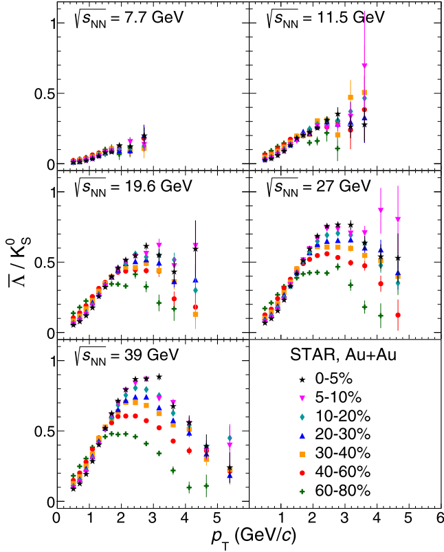
FIG. 29. \bar{\Lambda}/K_S^0 ratio as a function of p_T at midrapidity ( |y| < 0.5 ) in different centralities from Au + Au collisions at \sqrt{s_{NN}} = 7.7 –39 GeV. Errors are statistical only.
