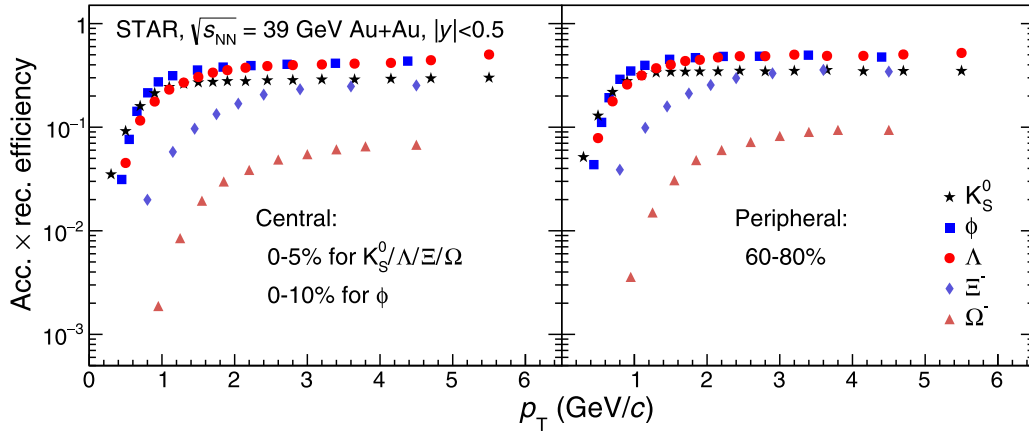
FIG. 3. Geometrical acceptance and reconstruction efficiency of various strange hadrons at midrapidity ( |y| < 0.5 ) in central (left) and peripheral (right) Au + Au collisions at \sqrt{s_{NN}} = 39 GeV. The branching ratios of measured decay channels are not taken into account here.
