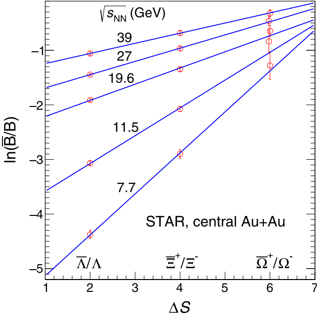
FIG. 25. Thermal model fitting to \ln(\bar{B}/B) vs \Delta S with a linear function to determine \mu_B/T_{\text{ch}} and \mu_S/T_{\text{ch}} for central Au + Au collisions at \sqrt{s_{\text{NN}}} = 7.7\text{--}39 GeV. The \bar{\Omega}^+/\Omega^- data points at 11.5 and 27 GeV are slightly shifted to the left for clarity.
