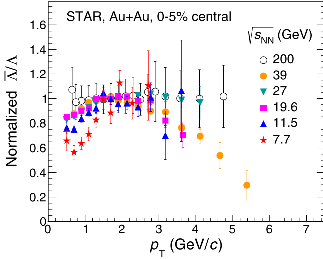
FIG. 22. Normalized \bar{\Lambda}/\Lambda ratio as a function of p_T from 0–5% central Au + Au collisions at different energies. The STAR results at \sqrt{s_{NN}} = 200 GeV [32] are shown as open circles for comparison. The errors are statistical only. All the ratios are normalized according to the average values inside the p_T range of [1.4, 2.0] GeV/c.
