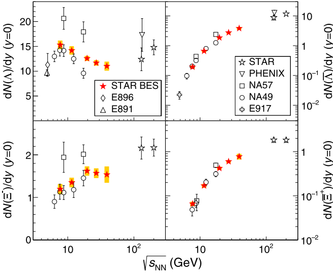
FIG. 19. Collision energy dependence of the \Lambda , \bar{\Lambda} , \Xi^- , and \bar{\Xi}^+ integrated yields, dN/dy , at midrapidity ( |y| < 0.5 ) in 0–5% central Au + Au collisions at \sqrt{s_{NN}} = 7.7 –39 GeV. \Lambda ( \bar{\Lambda} ) yields are corrected for weak decay feed-down. The orange shaded bands on the STAR BES data points represent the systematic errors. Also shown are the results from central Au + Au collisions at AGS [14,15,17,18], PHENIX [38] and STAR [29,31,32,37] and central Pb + Pb collisions at NA57 [26,27] and NA49 [24]. The rapidity ranges are |y| < 0.5 for NA57, PHENIX, NA49 \Xi^- ( \bar{\Xi}^+ ), and STAR \Lambda at 130 and 200 GeV, |y| < 0.75 for STAR \Xi^- at 130 and 200 GeV, |y| < 0.4 for AGS and NA49 \Lambda ( \bar{\Lambda} ). The \Lambda and \bar{\Lambda} results from AGS and PHENIX are inclusive, and those from NA49 and from STAR at higher energies are corrected for weak decay feed-down, while those from NA57 are not significantly affected by weak decay feed-down ( < 5\% for \Lambda and < 10\% for \bar{\Lambda} ). The E896, PHENIX, and NA57 8.7 GeV \bar{\Xi}^+ data points are slightly shifted to the right for clarity.
