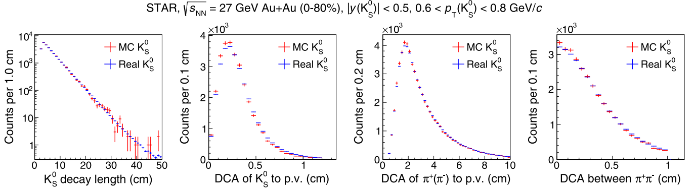
FIG. 4. MC and data comparison on K_S^0 topological variable distributions in Au + Au collisions at \sqrt{s_{NN}} = 27 GeV. A same set of loose selection cuts have been applied to both MC and data. The distributions of combinatorial backgrounds in data were estimated with the rotation method and subtracted, and then the resulting data distributions were scaled down to match with the MC statistics.
