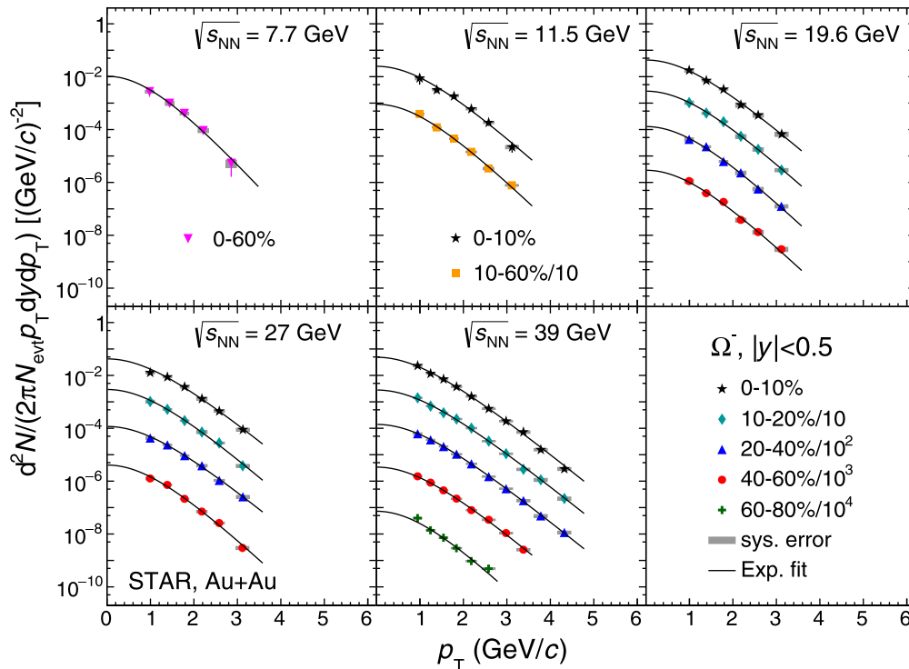
FIG. 10. The transverse-momentum spectra of \Omega^- at midrapidity ( |y| < 0.5 ) from Au + Au collisions at different centralities and energies ( \sqrt{s_{NN}} = 7.7\text{--}39 GeV). The data points are scaled by factors of 10 from central to peripheral collisions for clarity. The vertical gray bands represent the systematic errors, which are small hence the bands look like horizontal bars. The exponential function fit results are shown in the fit range and the low- p_T extrapolation range as solid lines for all centrality bins.
