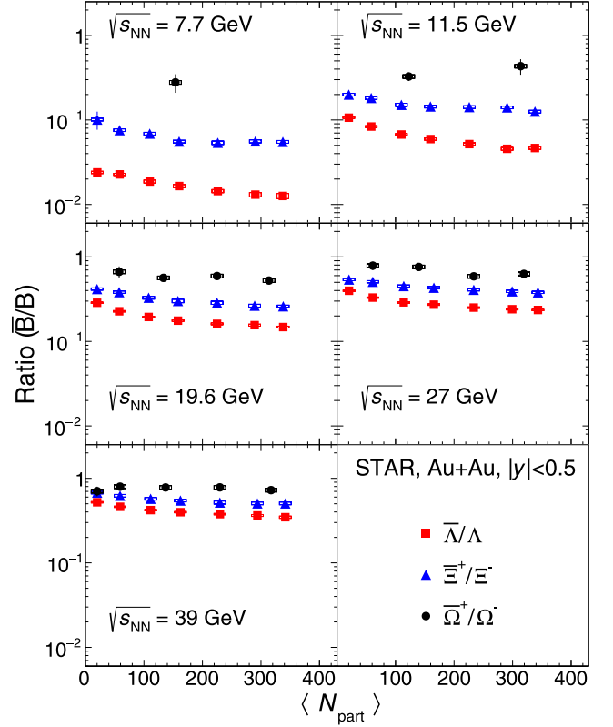
FIG. 20. The antibaryon-to-baryon ratios, \bar{\Lambda}/\Lambda , \bar{\Xi}^+/\Xi^- , and \bar{\Omega}^+/\Omega^- , as functions of \langle N_{part} \rangle from Au + Au collisions at \sqrt{s_{NN}} = 7.7 –39 GeV. The box on each data point denotes the systematic error.
