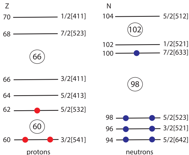
FIG. 2. Empirical single-particle levels near the proton and neutron Fermi surface for ^{160}\text{Pm} .
