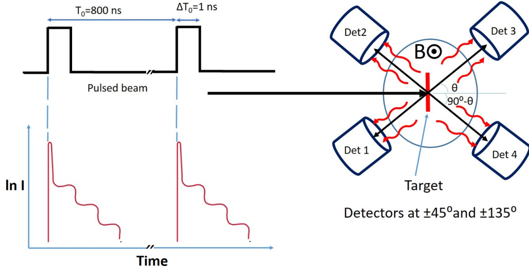
FIG. 1. Schematic drawing of the experimental arrangement of the TDPAD setup.
