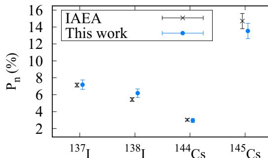
FIG. 7. Comparison of the BPT results ( \beta r P_n values) to the recommended IAEA values [14] obtained from previous direct measurements.
