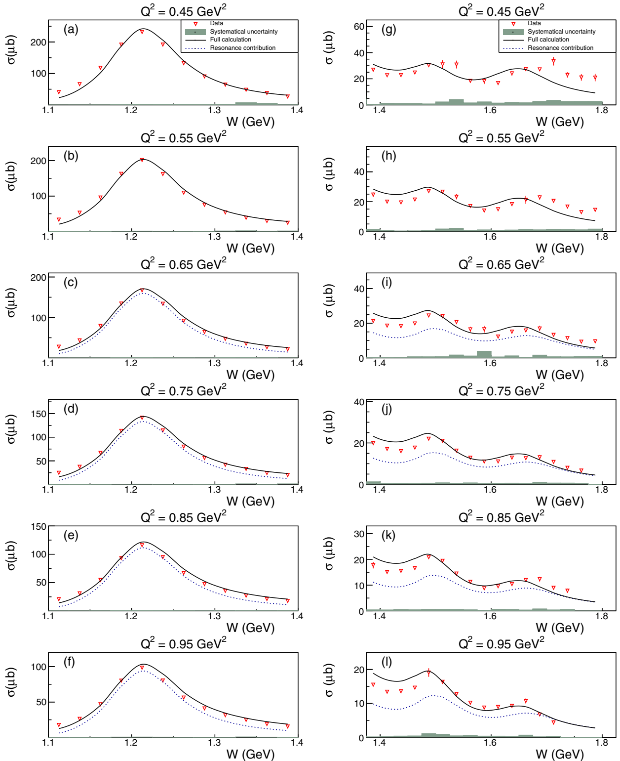
FIG. 17. Integrated \gamma_n p \rightarrow \pi^0 p' cross sections as a function of W in the first (left) and second and third (right) resonance regions for different values of Q^2 . The error bars, comparable with the symbol sizes, account for the statistical uncertainties only. Systematic uncertainties are shown by the shadowed areas. Model calculations from the JLab/YerPhi model [5] computed using electrocouplings and hadronic decay widths from fits to previous CLAS data [5,18,34] are shown as the black solid lines. The resonance-only contributions are shown as the blue dotted lines. The systematic uncertainties are shown by the shadowed areas at the bottom of the plots.
