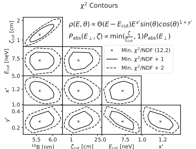
FIG. 6. Contours of \chi^2 in the parameter space of l_{10\text{B}} , \zeta_{\text{cut}} , E_{\text{cut}} , x' , and y' . On each subplot, the projection of the five-dimensional \chi^2 contours and the global minimum is shown.
