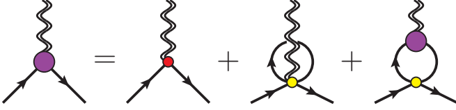
FIG. 2. Inhomogeneous Bethe-Salpeter equation for the dressed quark-graviton vertex.
