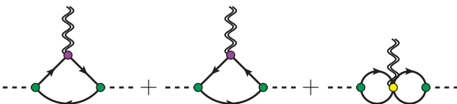
FIG. 3. Diagrams contributing to meson-graviton coupling.
