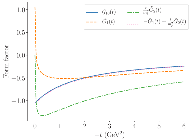
FIG. 10. The gravitational form factor \mathcal{G}_{10}(t) of the \rho meson, compared with the \rho axial form factors. The form factor \tilde{\mathcal{G}}_2(t) has been weighted by t/m_\rho^2 to make it comparable to the other form factors on the same plot.
