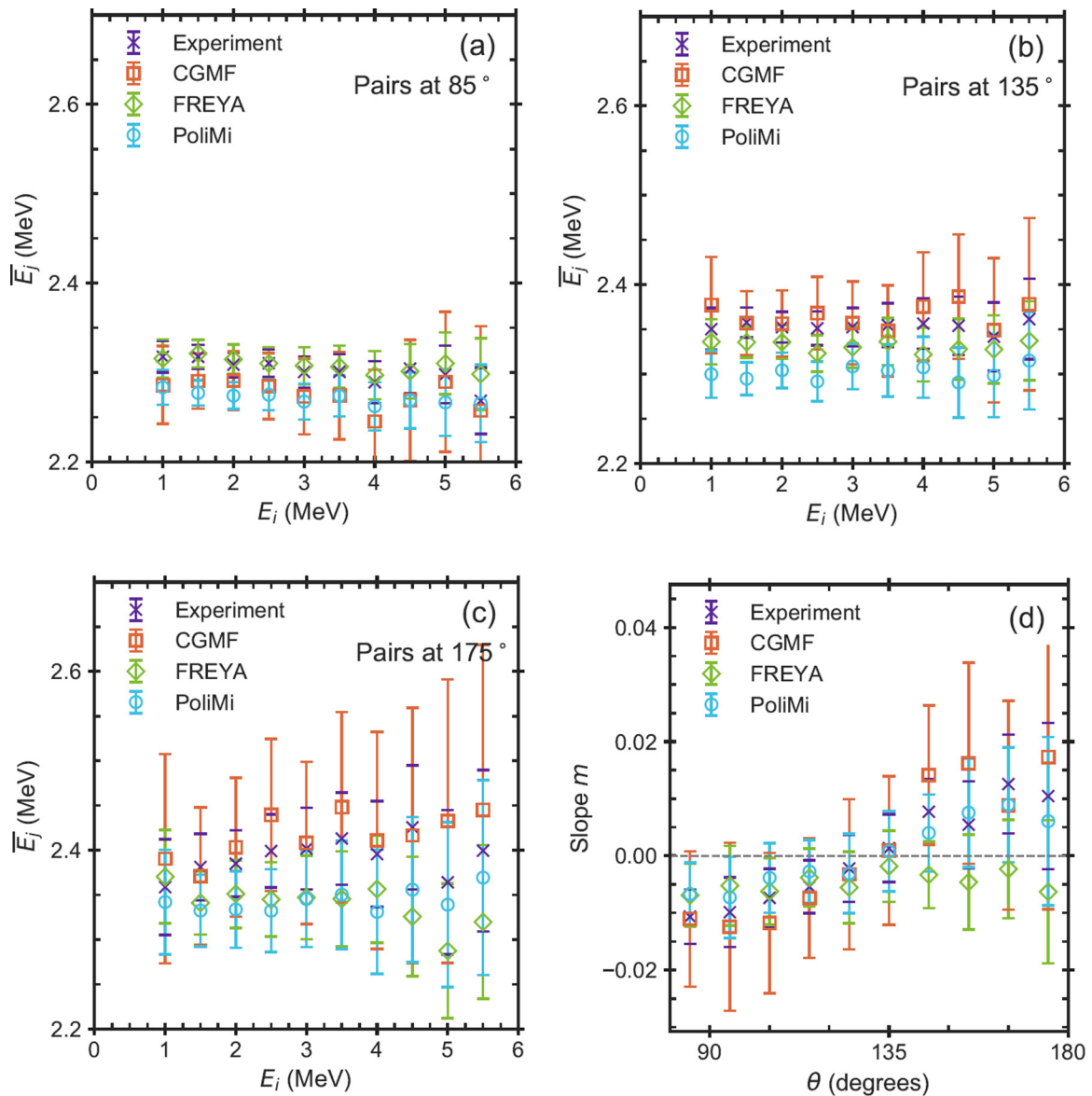
FIG. 10. Average correlated neutron energy \bar{E}_j for fixed energy E_i for detector pairs at (a) 85°, (b) 135°, and (c) 175°, and (d) slope of least-squares fit to E_j(E_i) at angles 85° and higher.
