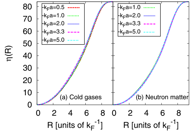
FIG. 6. Particle number \eta a distance R from the z axis, see Eq. (24), for the ground state and N = 84 for (a) cold gases and (b) neutron matter using the s -wave part of AV18. The legend conventions are the same as the ones employed in Fig. 5. The deviations between the behavior of different interaction strengths, or cold gases and neutron matter, are very small. Also, the differences between the two models for the neutron-neutron interactions are so minute that we chose to plot only one of them. An inspection of Fig. 5 reveals a characteristic behavior of the density, due to the presence of hard walls, at \rho \approx 6.0 k_F^{-1} . For R \simeq 6.0 k_F^{-1} , \eta \gtrsim 45 , meaning that we have approximately this number of particles in the bulk portion of the cylinder, where effects of the hard walls are mitigated.
