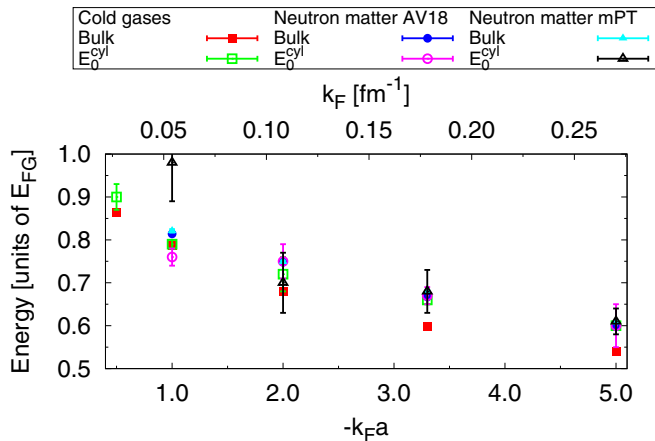
FIG. 3. Equation of state for cold atoms and low-density neutron matter. The bulk energies per particle for the cold gases, closed (red) squares, were obtained using the modified Poschl-Teller potential with k_F r_e = 0.05 . For neutron matter, the bulk energies per particle using the s -wave part of AV18 are denoted by closed (blue) circles, and the model using a modified Poschl-Teller potential with a^m = -18.5 fm and r_e^m = 2.7 fm is represented by closed (cyan) triangles. We also plot the fitted parameters E_0^{\text{cyl}} of Eq. (1) for cold gases and neutron matter ( s -wave part of AV18 and modified Poschl-Teller) with open symbols: (green) squares, (magenta) circles, (black) triangles, respectively. In the top x axis we plot the corresponding k_F for neutron matter.
