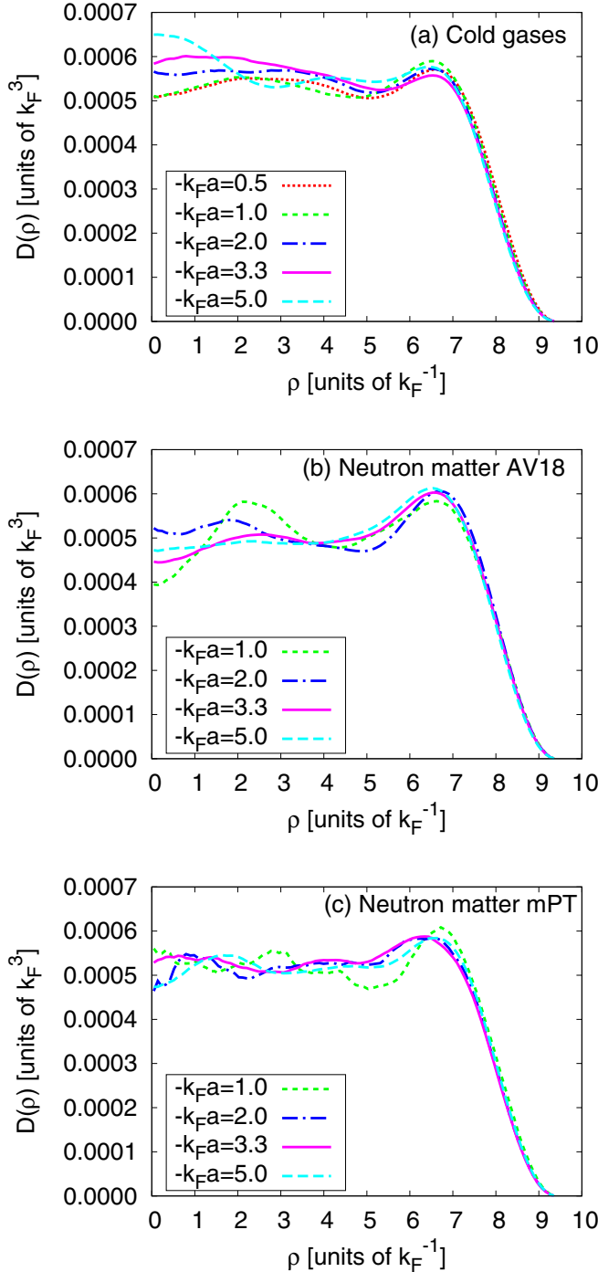
FIG. 5. Density profile of the ground state as a function of the radial coordinate \rho for N = 84 for (a) cold gases, (b) neutron matter using the s -wave part of AV18, and (c) the modified Poschl-Teller potential. The interaction strengths -k_F a = \{0.5, 1.0, 2.0, 3.3, 5.0\} correspond to the short-dashed (red) line, dashed (green) line, dashed-dotted (blue) line, solid (magenta) line, and long-dashed (cyan) line, respectively.
