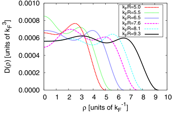
FIG. 1. Density profile of the free Fermi gas as a function of the radial coordinate \rho for N = 78 and several radii: 5.0k_F^{-1} long dashed (red) line, 5.5k_F^{-1} dashed (green) line, 6.5k_F^{-1} short dashed (blue) line, 7.6k_F^{-1} long dashed-dotted (magenta) line, 8.1k_F^{-1} dashed-dotted (cyan) line, and 9.3k_F^{-1} continuous (black) line. The number density was kept fixed at the free Fermi gas value, k_F^3/(3\pi^2) . Although the behavior close to \rho = \mathcal{R} is similar for all radii, due to the presence of the hard walls, the profile at the center of the cylinder, \rho \lesssim 2.0k_F^{-1} , can be quite different. In our simulations we employed \mathcal{R} = 9.3k_F^{-1} for N = 78 .
