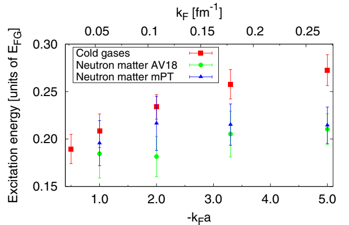
FIG. 4. Excitation energy per particle as a function of the interaction strength for both cold gases and neutron matter. The (red) squares denote the results for cold gases, i.e., using the modified Poschl-Teller potential with k_F r_e = 0.05 . For neutron matter, the results using the s -wave part of AV18 are denoted by (green) circles, and the model using a modified Poschl-Teller potential with a^m = -18.5 fm and r_e^m = 2.7 fm is represented by (blue) triangles. In the top x axis we plot the corresponding k_F for neutron matter. We can see that the excitation energies are comparable for -k_F a = 1 , however, when the density (or -k_F a ) increases, they start to differ.
