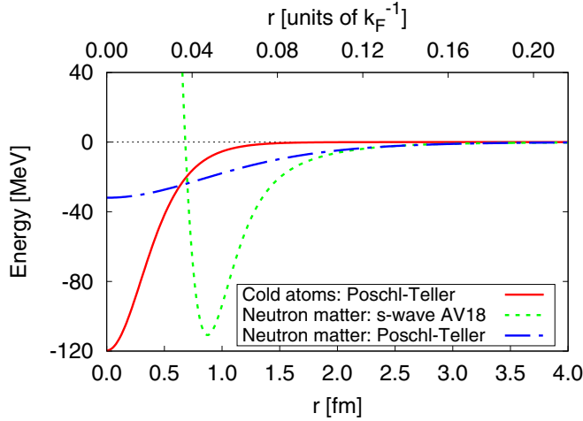
FIG. 2. Comparison between the pairwise interactions employed in this work for -k_F a = 1 . The continuous (red) line denotes the modified Poschl-Teller potential, Eq. (4), with k_F r_e = 0.05 , the dashed (green) line the s -wave component of AV18, and the dotted-dashed (blue) line stands for the modified Poschl-Teller potential tuned to reproduce a^{nm} = -18.5 fm and r_e^{nm} = 2.7 fm. The top x axis displays the distances in units of k_F^{-1} , considering the number density to be the same as the free Fermi gas, n = k_F^3/(3\pi^2) .
