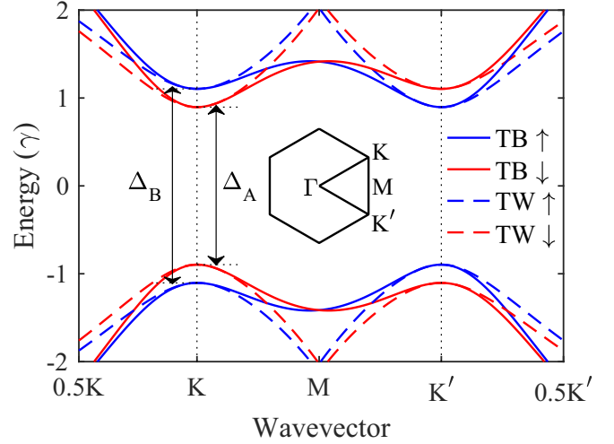
FIG. 1. Typical band structure of monolayer TMD near the band gap obtained using the full TB (solid lines) or TW Hamiltonian (dashed lines) for \gamma = \Delta = 50\lambda . Blue and red lines show spin-up ( s = 1 ) and -down ( s = -1 ) bands, respectively. The inset shows the BZ and its high symmetry points.
