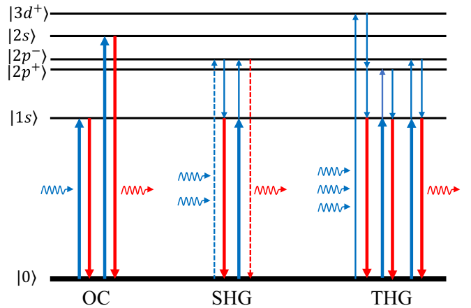
FIG. 3. Sketch of exciton energy levels at the K valley with the dominant transition paths (solid/dashed arrows) for the first resonances of OC, SHG, and THG spectra. Dashed arrows represent the TW-enabled transitions, see Fig. 2. Red arrows indicate transitions that relaxes the system to its ground state.
