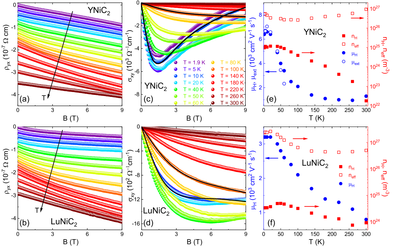
FIG. 4. [(a) and (b)] Magnetic-field dependence of Hall resistivity \rho_{yx} in \text{YNiC}_2 (a) and \text{LuNiC}_2 (b). The plots have been vertically shifted for clarity and the vertical scale applies to the plot for corresponding to T = 1.9 K. [(c) and (d)] Hall conductivity \sigma_{xy} in \text{YNiC}_2 (c) and \text{LuNiC}_2 (d). The black solid lines are representative fits to the experimental data with Eq. (9). [(e) and (f)] The results of the analysis of Hall resistivity and conductivity: mobilities \mu_H , \mu_{\text{ext}} and concentrations n_H , n_{\text{eff}} plotted as a function of temperature for \text{YNiC}_2 (e) and \text{LuNiC}_2 (f). The legend for (a), (b), (c), and (d) is displayed in panel (c).
