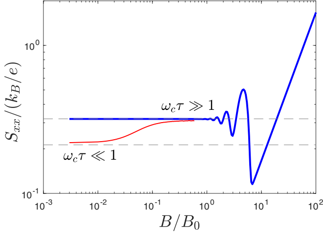
FIG. 5. The Seebeck coefficient S_{xx} of a three-dimensional Dirac/Weyl semimetal as a function of magnetic field B . The plot shows the result in the dissipationless limit (thick blue line) and the semiclassical result (thin red line) corresponding to a scattering time \tau = 50(v_F n_0^{1/3})^{-1} . The labeled dashed lines show the value of Eq. (41) in the limits of \omega_c \tau \ll 1 and \omega_c \tau \gg 1 , respectively. The temperature is taken to be T = 0.1 \hbar v_F n_0^{1/3} / k_B . In both plots, the units of magnetic field are B_0 = \hbar n_0^{2/3} / e , and units of \alpha_{xy} are \alpha_0 = e k_B n_0^{1/3} / \hbar . The linear increase in S_{xx} with B in the extreme quantum limit is described in detail in Ref. [13].
