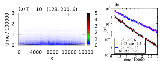
FIG. 9. (a) Normalized energy \mathcal{E}(x, t) for the system with very large value z = 3413 . Period of the source T = 10 . (b) Exponential decrease of the energy from the central region.
