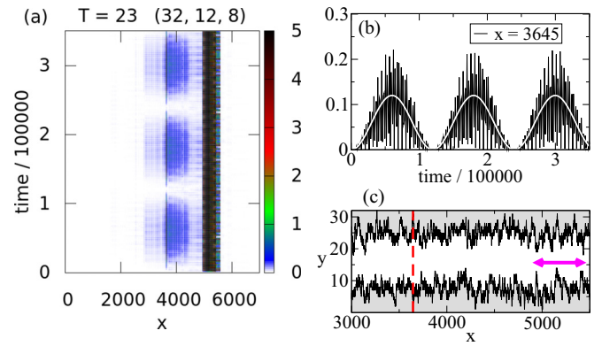
FIG. 5. (a) Localized phonon observed in a narrow and strongly disordered sample. The size of the sample is 32 \times 10240 , disorder h = 8 and correlation length l_c = 12 ( z = 78.8 ). Source is located at x = 5120 and period of the source is T = 23 . Small portion of energy tunnels from bottleneck region and excites periodically the resonance localized at x \approx 3645 . (b) The time evolution at energy E(x = 3645, t) . White solid line is given by Eq. (7) with \omega - \omega_R = 5.24 \times 10^{-5} . (c) The detail of the structure. Here vertical dashed line shows the position of the localized state and magenta arrow indicates the region where the injected energy is trapped.
