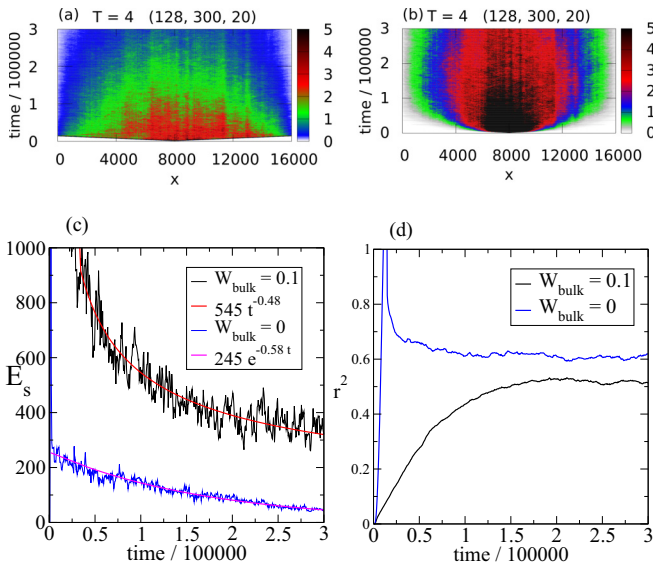
FIG. 10. Comparison of sample without and with bulk disorder W_{\text{bulk}} = 0.1 . Normalized energy \mathcal{E}(x, t) for (a) W_{\text{bulk}} = 0 and (b) W_{\text{bulk}} = 0.1 . (c) Bulk disorder changes the time dependence of the energy E_s(t) from exponential decrease to the power law. This suggests that diffusion is apparently more robust when bulk disorder is present. (d) r^2 for system with and without bulk disorder.
