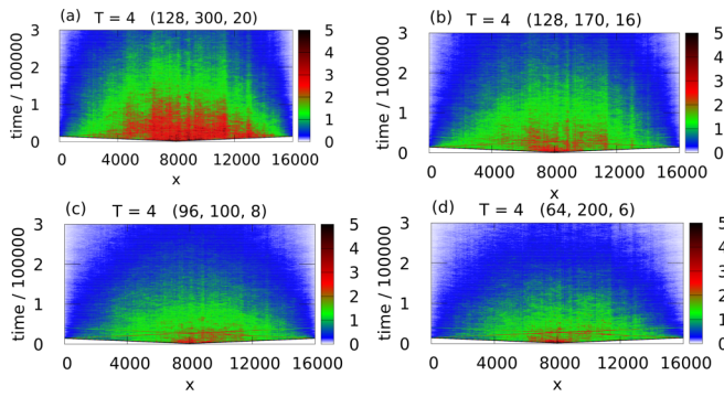
FIG. 6. Normalized energy \mathcal{E}(x, t) for four systems with different values of (d, l_c, h) but similar value of z = l_c^{1/2} d^{3/2} / h \approx 1200 . Period of the source T = 4 . Similarity of transport regimes in all four samples is supported also by calculation of r^2 shown in Fig. 7(a).
