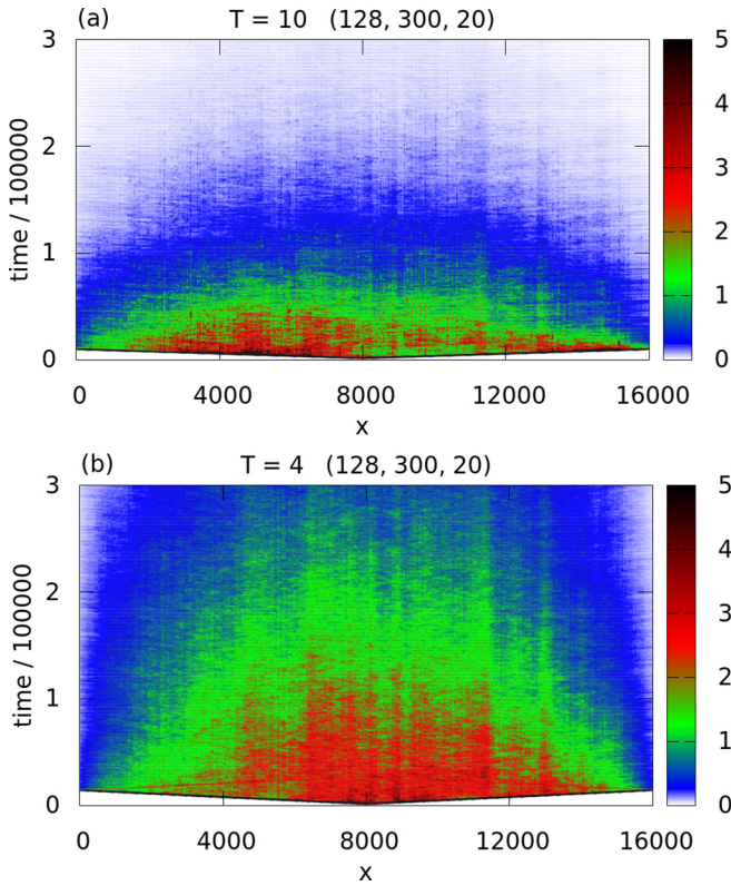
FIG. 4. Space and time evolution of normalized energy \mathcal{E}(x, t) in sample 128 \times 16000 with l_c = 300 and h = 20 ( z = 1253 ) for periods (a) T = 10 and (b) T = 4 . Note the similarity of panels for the period T = 10 with that shown in Fig. 3.
