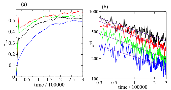
FIG. 11. (a) r^2 calculated for four different samples which differ by realizations of surface disorder. The size is 128 \times 16000 , l_c = 200 and h = 30 ( z = 682 ). Results give us some information about the statistical properties of calculated quantities. (b) Time evolution of the energy E_s(t) in the center behaves as E(t) \sim t^{-\alpha} with exponent \alpha \sim 0.32-0.37 .
