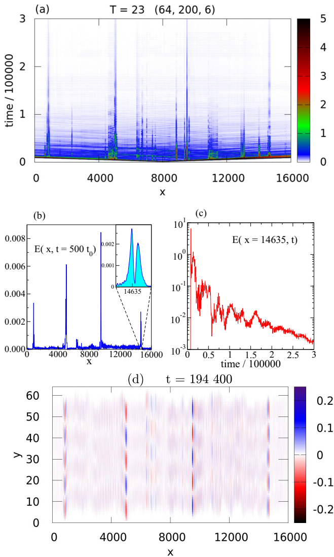
FIG. 2. (a) Space and time evolution of normalized energy \mathcal{E}(x, t) in the weakly disordered sample of size 64 \times 16000 . Period of the source T = 23 . Three length parameters, (d, l_c, h) = (64, 200, 6) are given in the title, corresponding to z = 1206 . A set of resonances excited by the external source is clearly visible, corresponding to localized phonons. (b) The space distribution of the energy at time t = 500t_0 ( t_0 = 555.55 ). Inset shows detail of the resonance at x = 14635 . (c) Time evolution of the energy at the position of resonance at x = 14635 . (d) Snapshot of u(x, y) at time t = 194400 offers another method to identify resonances showed in panels (a) and (b). Please note different scale on the horizontal and vertical axes.
