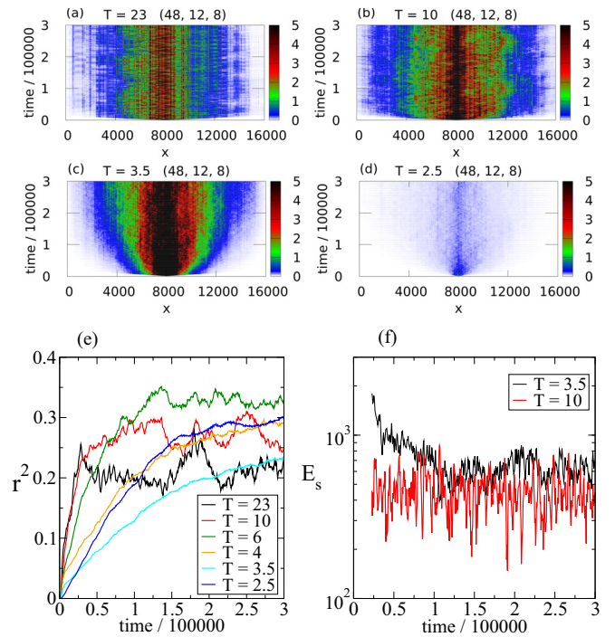
FIG. 8. Localization of phonons in strongly disordered system 48 \times 16000, l_c = 12 and h = 8 ( z = 144 ). Panels (a)–(d) show the normalized energy \mathcal{E}(x, t) for periods T = 23, 10, 3.5 and 2.5 . (e) time evolution of r^2 , (f) the energy E_s in the central region for periods T = 10 and T = 3.5 .
