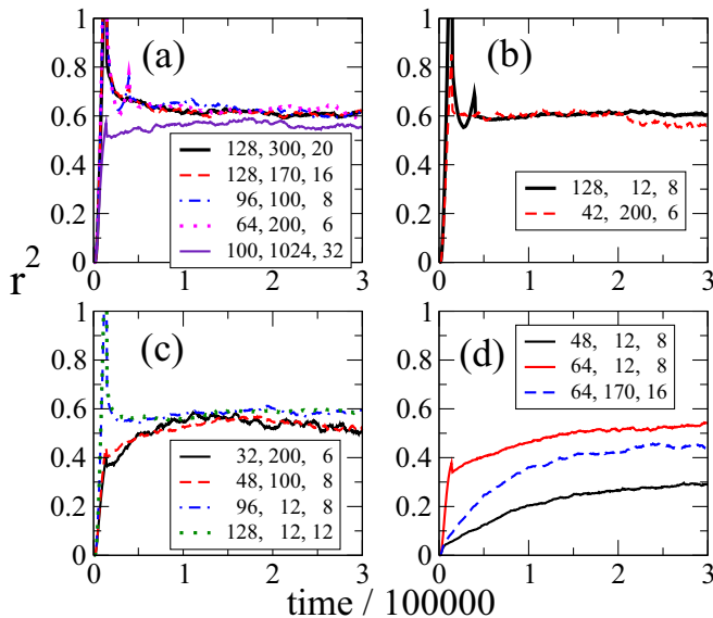
FIG. 7. r^2(t) for various systems illustrating universality. Period of the source T = 4 for all samples [40]. Data confirm that the limiting value of r_s^2 = \lim_{t \rightarrow \infty} r^2 depends only on single parameter z and decreases when z decreases. The universality is clearly visible in (a) where r^2 for four different systems with z \approx 1200 converge to the same limiting value. Similarly, in (b), z \approx 630 and in (c) z \approx 420 . Panel (d) show data for systems with much smaller values of z which exhibit the phonon localization (dashed line corresponds to system where bottleneck effect dominates to make transmission more difficult).
