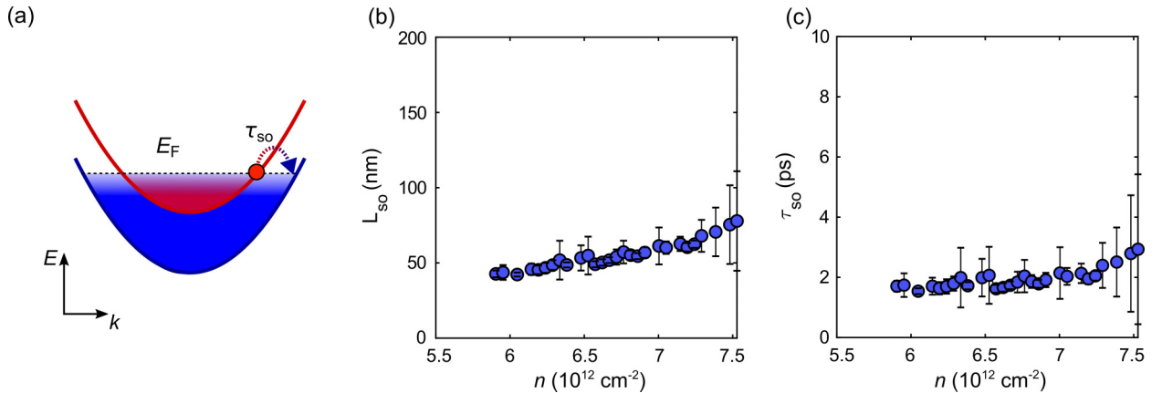
FIG. 4. Spin relaxation properties of electrons in bilayer \text{MoS}_2 . (a) Energy-dispersion schematic illustrating spin relaxation due to intervalley spin-flip process. Different colors represent electron populations of different spin orientations. Spin relaxation length L_{so} (b) and time \tau_{so} (c) as a function of electron density ( T = 2 \text{ K} ), obtained from fitting the magnetoconductivity data to Eq. (1). The spin relaxation length increases with electron density, while the spin relaxation time is independent of the electron density.
