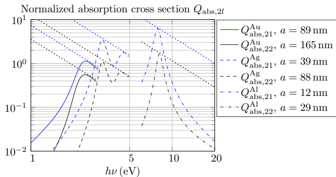
FIG. 4. Normalized dipole and quadrupole absorption cross sections Q_{\text{abs},2l}^{\text{Ax}} , l = 1, 2 , for a sphere made of gold (Au), silver (Ag), and aluminum (Al), and where the radius a has been tuned to match the condition (60) for optimal absorption; see also Fig. 3. The almost tangent optimal bounds are plotted as dotted lines. Here, the background is lossless with \epsilon_b = 1 .
