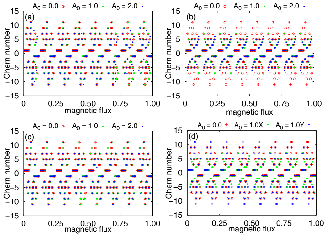
FIG. 5. The ground-state Chern number of the Floquet Hofstadter butterfly spectrum for the kagome lattice. Laser frequency is fixed at an off-resonance value of \Omega = 9.0 . (a) Circularly polarized light with A_0 = 0.0, 1.0, 2.0 . (b) Linearly polarized light along x ( \alpha = 0.0 ), A_0 = 0.0, 1.0, 2.0 . (c) Linearly polarized light along y ( \alpha = \pi/2 ), A_0 = 0.0, 1.0, 2.0 . (d) Linearly polarized light A_0 = 1.0 along x and y as a comparison. The calculations are done with nine Floquet copies. The magnetic flux is defined as \phi = p/8q , with p ranging from 1 to 8q - 1 and q \leq 13 .
