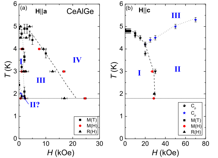
FIG. 7. T - H phase diagrams for CeAlGe single crystals. Different phases are marked with Roman numerals. Horizontal dashed lines indicate the temperature limit of our measurements. (a) \mathbf{H}||\mathbf{a} . Phase III represents canted moment phase of the spin-flop transition. Phase IV represents a spin-flop to a partially saturated moment ( < 1 \mu_B ) phase. (b) \mathbf{H}||\mathbf{c} .
