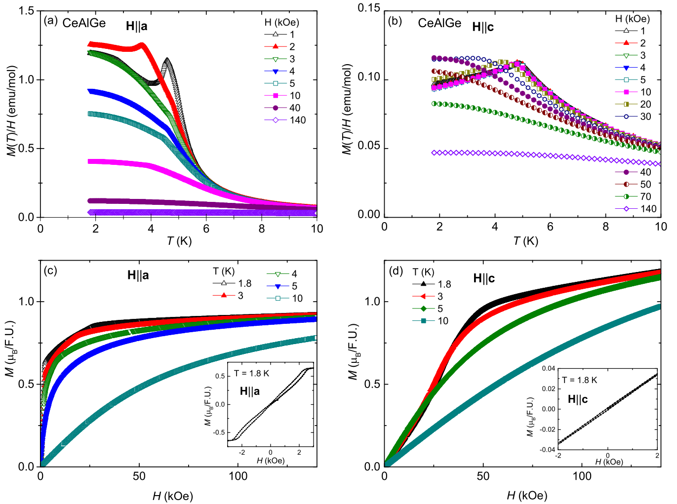
FIG. 3. (a) and (b) Temperature-dependent magnetization of CeAlGe at constant magnetic fields for \mathbf{H}\parallel\mathbf{a} and \mathbf{H}\parallel\mathbf{c} , respectively. (c) and (d) Field-dependent magnetization of CeAlGe single crystal for \mathbf{H}\parallel\mathbf{a} and \mathbf{H}\parallel\mathbf{c} , respectively.
