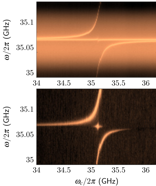
FIG. 3. Power reflection from the cavity (top panel) and electron dc conductivity response (bottom panel) versus the cyclotron frequency of electrons \omega_c and frequency of MW excitation \omega measured at T = 0.2 K for electron surface density n_s = 8.0 \times 10^7 \text{ cm}^{-2} and input MW power P = -9 dBm.
