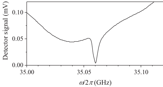
FIG. 2. Spectrum of power reflection from the filled cavity resonator measured at T = 0.2 K without electrons and an input MW power P = 0 dBm.
