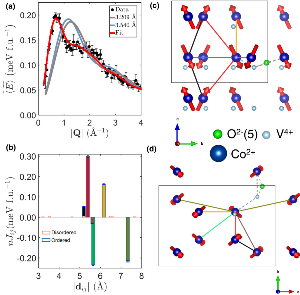
FIG. 7. (a) |Q| dependence of the background-subtracted first moment \langle \widetilde{E} \rangle as measured on MARI at T = 5 K with an E_i = 15 meV integrated over E = [2, 8] meV. A fit to the first moment sum rule [Eq. (11)] reveals that only six distances |d_{ij}| out to 7.5 \text{\AA} possess non-negligible nJ_{ij} values as illustrated in (b), and summarized in Table III. For the purposes of comparison, distances present only in the ordered and disordered atomic arrangements are distinguished by purple and dark pink outline colors, respectively. Distances with non-negligible nJ_{ij} contributions have a face color corresponding to the illustration of the corresponding six interactions along the (c) bc and (d) ac planes of the \alpha\text{-CoV}_3\text{O}_8 unit cell. Both nonbridging oxygen atoms have been excluded and \text{V}^{4+} ions have been reduced in size for the purposes of clarity. Two particular distances, 3.209 \text{\AA} and 3.540 \text{\AA} , are absent as noted in (a), corresponding to nearest neighbor and bridging metal site distances, respectively.
