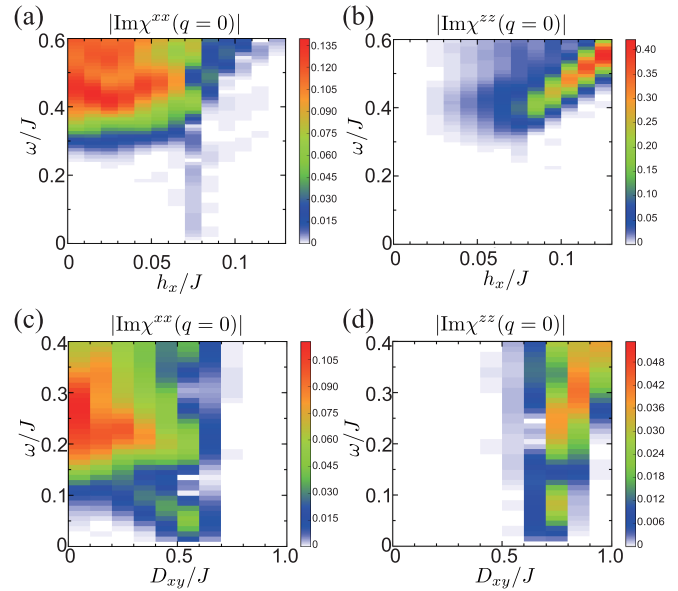
FIG. 6. Dynamical susceptibility (a) \chi^{xx}(q = 0) and (b) \chi^{zz}(q = 0) for the XXZ model ( \Delta = 1.9 ) with staggered x field and (c) \chi^{xx}(q = 0) and (d) \chi^{zz}(q = 0) for the XXZ model ( \Delta = 1.6 ) with XY anisotropy.
