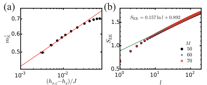
FIG. 2. (a) Log-log plot of m_N^z as a function of h_{x,c} - h_x . (b) Semi-log plot of entanglement entropy for a finite interval S_{\text{EE}} as a function of the size of the interval l at h_x = h_{x,c} . M is the bond dimension of MPS (see the Appendix).
