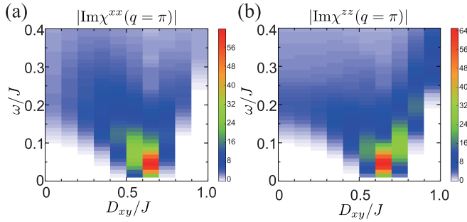
FIG. 5. Dynamical susceptibility (a) \chi^{xx}(q = \pi) and (b) \chi^{zz}(q = \pi) for the XXZ model ( \Delta = 1.6 ) with XY anisotropy. Both \chi^{xx} and \chi^{zz} diverge at the transition point D_{xy}/J = 0.6 .
