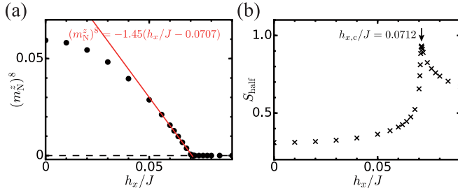
FIG. 3. Plot of (a) (m_N^z)^8 and (b) half-infinite entanglement entropy S_{\text{half}} as a function of h_x .
