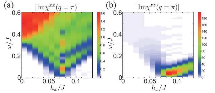
FIG. 4. Dynamical susceptibility (a) \chi^{xx}(q = \pi) and (b) \chi^{zz}(q = \pi) for the XXZ model ( \Delta = 1.9 ) with staggered x field. The dominant low energy excitation in the low (high) h_x phase corresponds to \chi^{xx} ( \chi^{zz} ). We see that \chi^{zz} diverges at the transition point h_x/J \simeq 0.071 while \chi^{xx} does not.
