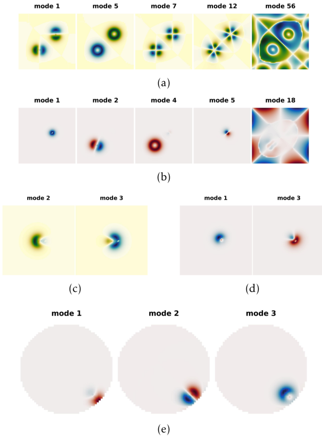
FIG. 8. Eigenmodes associated to the \theta variable. The color code is the same as in Fig. 7. Additional mode profiles can be found in Ref. [21] for each of the following mechanisms. [(a) and (b)] Internal and collective modes of two coupled skyrmions on a 50 \times 50 lattice at A and S . [(c) and (d)] Modified internal modes for the collapse on a defect at A and S . (e) Modified internal modes for the escape through a curved boundary at S .
