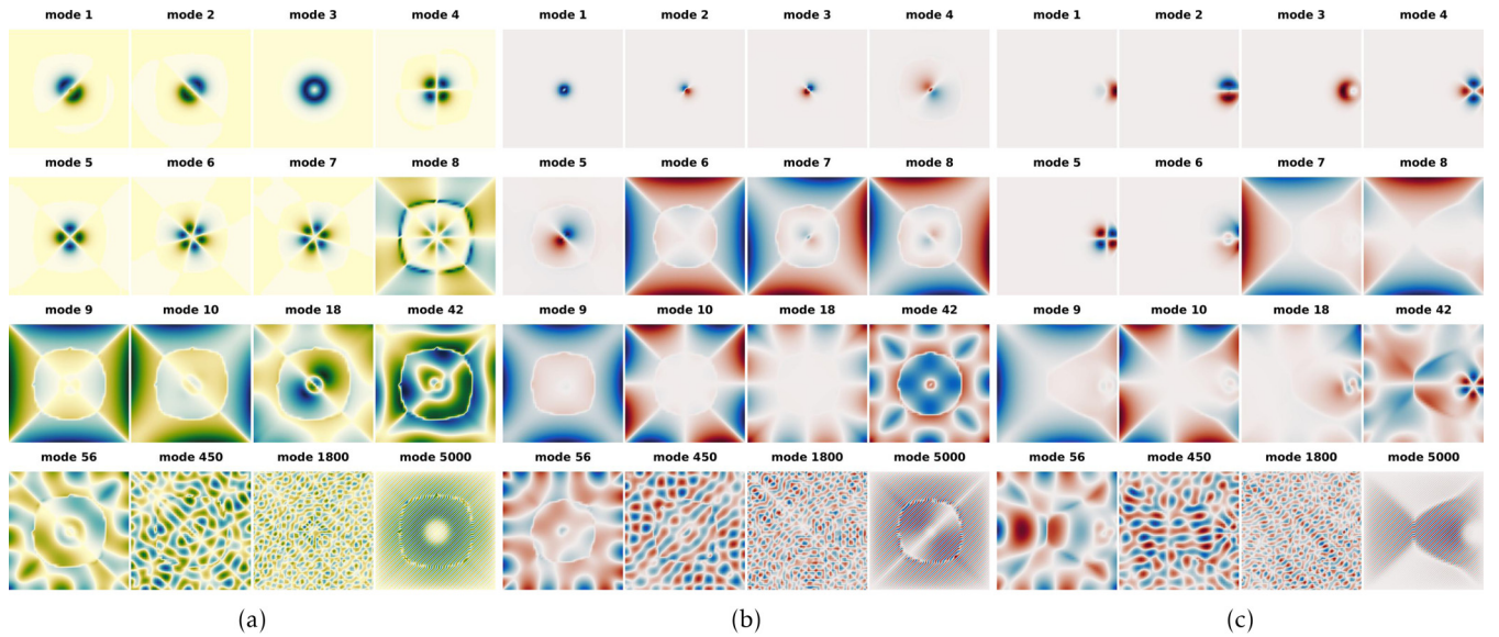
FIG. 7. Eigenmodes associated to the \theta variable for a single skyrmion in a simulated system of 50 \times 50 spins. The blue and green color scheme is associated with metastable states and the blue and red one with saddle points. Negative amplitudes are plotted in blue and positive ones in green/red. The range of the color map is adjusted on each plot so that zero-amplitude fluctuations coincide with white. Modes are designated via the i -index of the corresponding ordered eigenfrequencies of Fig. 6. (a) Metastable single-skyrmion state with localized modes i = 1, \dots, 7 and collective modes i > 7 . (b) Saddle point of the collapse with localized modes i = 1, \dots, 5 and collective modes i > 5 . (c) Saddle point of the escape with localized modes i = 1, \dots, 6 and collective modes i > 6 .
