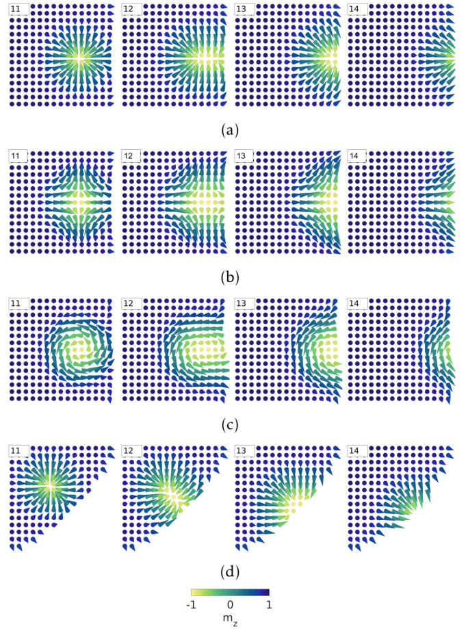
FIG. 3. Spin maps of the escape mechanisms. The conventions are the same as in Fig. 2. On all the subfigures, the saddle point is im. 11, which is the state where the skyrmion sits tangent to the boundary. (a) Néel skyrmion. (b) Antiskyrmion. (c) Bloch skyrmion. (d) Néel skyrmion escaping through a curved boundary.
