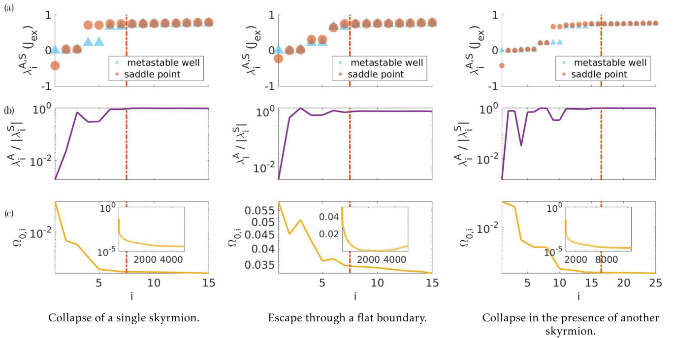
FIG. 6. For the first few eigenvalues of each annihilation mechanism, we show the following: (a) eigenvalues at A and S , (b) ratio of individual eigenvalues in semilogarithmic scale, and (c) \Omega_{0,i} in semilogarithmic scale. The inset figure shows all eigenvalues. The red dotted line marks the separation between localized and collective eigenmodes. The x axis is the same for all subfigures.
