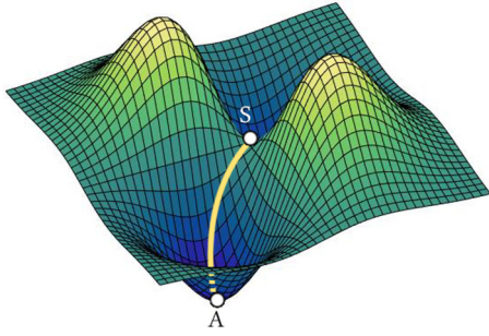
FIG. 1. Typical energy surface of a system possessing a metastable local minimum A and a stable global minimum M separated by a saddle point S . The reaction coordinate is represented by a yellow line and corresponds to the path of minimum energy connecting A , S , and M .
