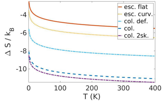
FIG. 9. Calculated change in configurational entropy induced when the system goes to the saddle point \Delta S/k_B = \frac{S_S - S_A}{k_B} as defined in Eq. (10) over a broad range of temperatures for all mechanisms. The highest entropic barrier corresponds to the most negative \Delta S , i.e., the collapse involving a second skyrmion.
