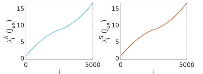
FIG. 5. All energy curvatures at A (in blue) and S (in red) ordered by increasing amplitudes for the case of the collapse of a single skyrmion. The other mechanisms exhibit the same profiles which we interpreted as the dispersion of spin-wave excitations, with the exception of the mechanism of spin of spin-wave excitations. These are found below the main curve and are shown on Fig. 6(a).
