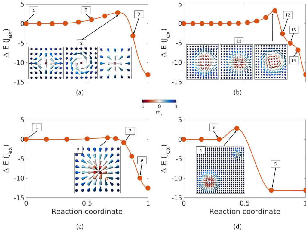
FIG. 4. Interpolated energy profiles along the normalized reaction coordinate. Each dot corresponds to an image of the system on the energy surface. The insets show a closeup of the spin configuration at the saddle point. (a) Collapse of a single skyrmion. The energy increases slowly as the skyrmion shrinks (ims. 1–8). Past the barrier top (im. 8), it annihilates by breaking the radial symmetry which is accompanied by a brutal decrease in the energy. (b) Escape through a flat boundary. The energy rises as the skyrmion gets closer to the edge (ims. 9–11). The top of the barrier is the state tangent to the boundary (im. 11). Past that point, the skyrmion disappears through the edge. This is accompanied by a rapid drop in the energy, with a notable slowdown halfway through the process as half the skyrmion has disappeared (im. 13). (c) Collapse in the presence of a single non-magnetic defect. The skyrmion shrinks in size as the core moves towards the defect. This costs very little energy (ims. 1–5). Past the saddle point, the skyrmion collapses on the defect. (d) Collapse in the presence of another skyrmion. The skyrmions get closer to each other, which at first costs little energy (ims. 1–3) until a critical distance is reached where the collapse of the upper skyrmion is initiated. The saddle point is the same as that of the first mechanism for the upper skyrmion, while the other remains stable (im. 4).
