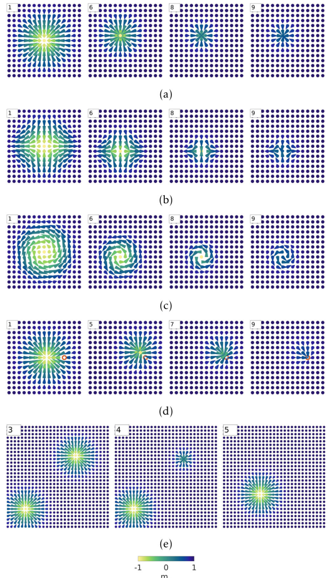
FIG. 2. Spin maps of the collapse mechanisms. The index in the top left-hand corner corresponds to the image index of the GNEB method. The saddle point corresponds to the state preceding the flipping of the core spin. (a) Néel skyrmion. (b) Antiskyrmion. (c) Bloch skyrmion. (d) Néel skyrmion in the presence of a nonmagnetic defect. (e) Néel skyrmion in the presence of a second skyrmion.
