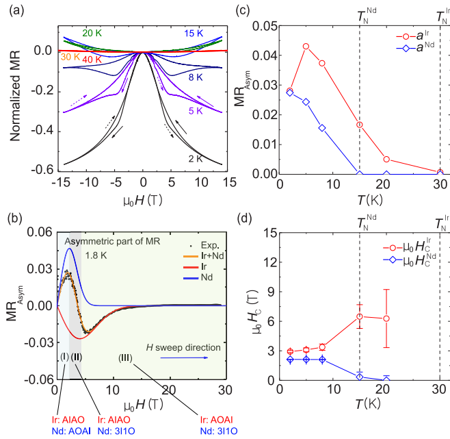
FIG. 5. (a) Normalized MR at various temperatures with H \parallel [111] . (b) Asymmetric component of the sweep-up MR at 1.8 K (positive H ). The colored region with roman numerals corresponds to the represented spin structures. The red (blue) and orange solid lines indicate the hysteretic part of Ir (Nd) domain switching from Eq. (2) and its total contribution to both Nd and Ir, respectively. (c) Quantified fit parameters a extracted from Eq. (2), where red empty circles (blue empty diamonds) indicate the contribution of hysteretic behavior from Ir (Nd) domain switching. (d) Red empty circles and blue empty diamonds are the coercive fields of the Ir domain and Nd spins, respectively, from MR. At 30 K, the asymmetric MR becomes too small to obtain reliable values of the coercive field.
