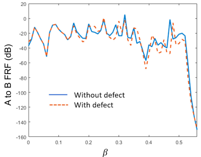
FIG. 10. Frequency response function of a topological wave guide with and without defect at the Dirac frequency for varying contrast \beta .
