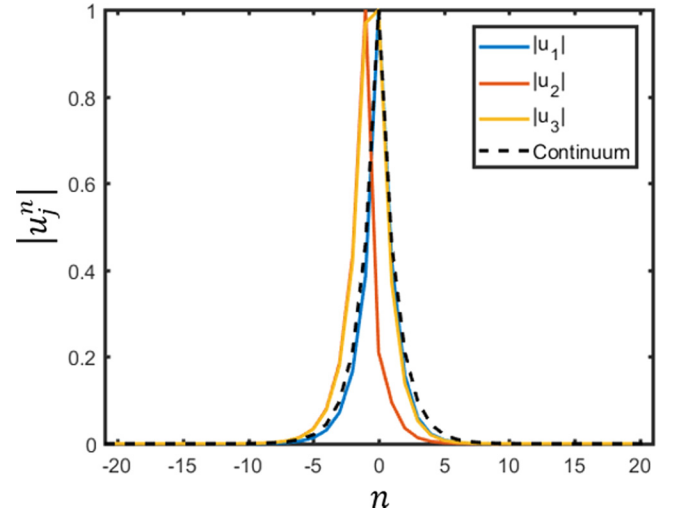
FIG. 6. Decay profiles of the Stoneley wave at q_x = 0 calculated numerically (solid) and asymptotically (dashed). Each solid line corresponds to one mass per unit cell indexed with the subscript j ; there are nine similar lines in total but only three of them are shown for clarity. Integer n indexes unit cells: n = 0 corresponds to the unit cell at the interface, n > 0 (resp. < 0 ) to unit cells above (resp. below) the interface.
