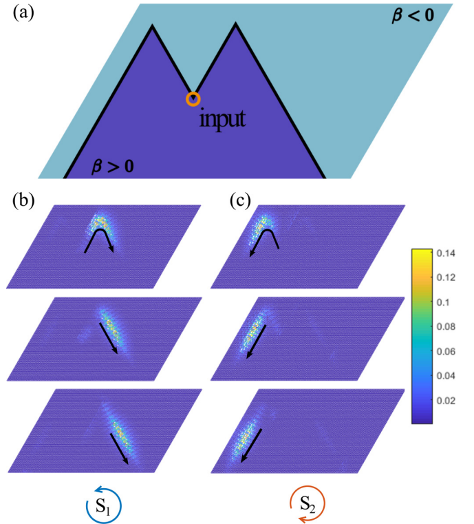
FIG. 7. Immunity to backscattering at corners ( 60 - 120^\circ ): (a) geometry; (b) snapshots of the displacement amplitude as a color map for a positively polarized excited wave at t = 200, 250, 300 respectively; (c) same as (b) for a negatively polarized excited wave.
