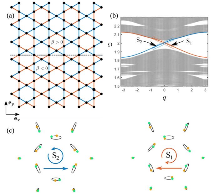
FIG. 5. Bulk and edge spectra of a finite sample of 40 unit cells under free (resp., periodic) boundary conditions in the y direction (resp., x direction) with \beta = 0.2 for y > 0 and \beta = -0.2 for y < 0 : (a) geometry, (b) diagram: continuous lines correspond to the numerical result and circles correspond to the asymptotic result [Eqs. (29) and (30)], (c) mass trajectories of interface states for q = \pm 0.5 .
