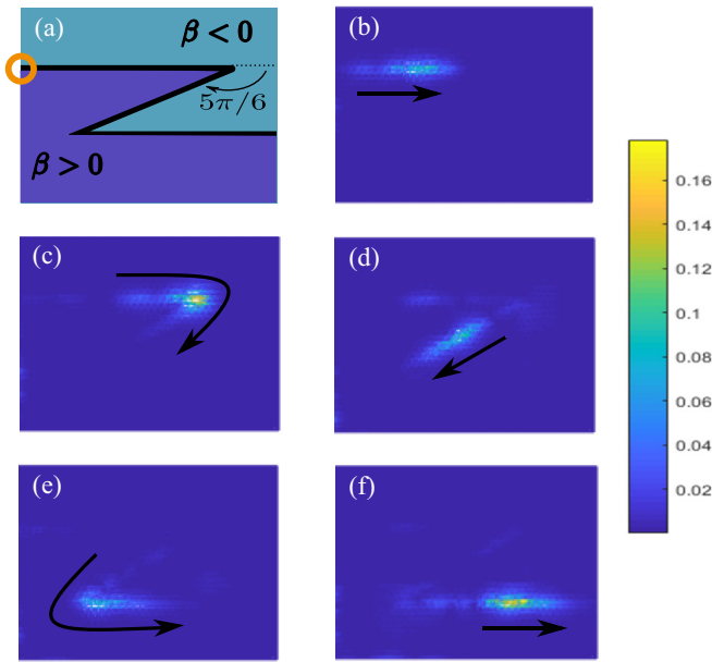
FIG. 8. Immunity to backscattering at corners ( 30 - 150^\circ ): (a) geometry; (b) snapshots of the displacement amplitude as a color map for a positively polarized excited wave at (b) t = 150 , (c) t = 250 , (d) t = 350 , (e) t = 450 , and (f) t = 550 .
