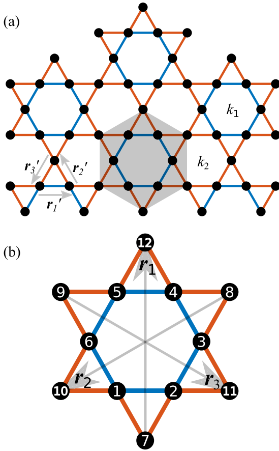
FIG. 1. The perturbed kagome lattice (a) and a magnified view of its unit cell (b). Edges are springs of constant k_1 if blue, k_2 if red.
