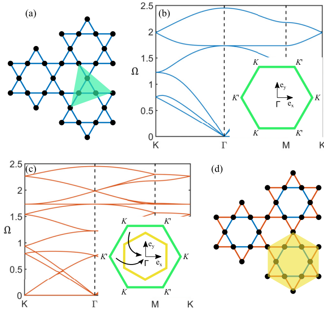
FIG. 2. The kagome lattice: (a) homogeneous configuration, (b) its dispersion diagram featuring two Dirac cones between the fifth and sixth bands at K and K' , (c) folded dispersion diagram featuring a double Dirac cone at the \Gamma point, (d) the corresponding perturbed configuration. Note that diagram (c) correspond to the lattice in (d) only in the limit k_1 = k_2 .
