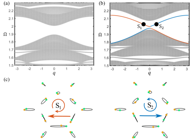
FIG. 4. Bulk and edge spectra of a finite sample of 20 unit cells under free (resp., periodic) boundary conditions in the y direction (resp., x direction) for \beta = 0.1 (a) and \beta = -0.1 (b). In the latter case, edge modes exist and the corresponding mass trajectories are illustrated on (c) for q = \pm 0.5 .
