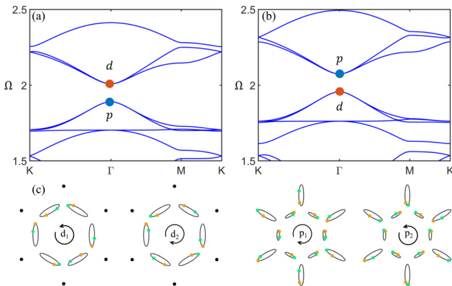
FIG. 3. Band inversion: dispersion diagrams for \beta = 0.1 (a) and \beta = -0.1 (b). As \beta \neq 0 , the fourfold degeneracy breaks into two twofold degeneracies. The mass trajectories of the degenerate eigenstates are illustrated in (c) along with their polarizations: a solid green dot corresponds to the initial position of the mass and an orange dot corresponds to the position at a later small time. Black dots correspond to nonmoving masses.
