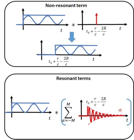
FIG. 2. Schematic representation of nonresonant and resonant terms in Eq. (10).
