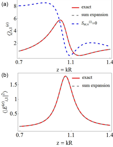
FIG. 1. (a) Dipolar electric partial scattering efficiency Q_1^{(e)} = \frac{6}{z^2} |T_1^{(e)}|^2 and (b) averaged square modulus of the internal electric field with |\mathbf{E}_0| = 1 for an \varepsilon = 16 spherical scatterer in air: exact calculations (red solid curve); (a) Eq. (4) with M = 100 poles and (b) Eq. (5) with M = 10 poles (gray dashed line); (a) Eq. (4) with M = 100 while assuming S_{nr,n}^{(e,h)} = 0 (blue dashed curve).
