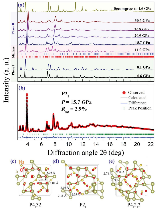
FIG. 3. (a) The background-subtracted diffraction patterns of Na 3 Ir 3 O 8 at high pressures and room temperature. The colored backgrounds represent the changes in the diffraction patterns. A clear structural phase transition takes place above 8.1 GPa where additional peaks appear in the diffraction pattern. The positions of the Bragg reflections of the low-pressure (phase I) and high-pressure (phase II) phases within the mixture pattern, at the pressure of 11.0 GPa are marked by vertical sticks in blue and red, respectively. The structure goes back to ambient pressure phase when pressure is released to 4.6 GPa. (b) Observed and Rietveld refined profiles within space group P2_1 at 15.7 GPa (phase II). The solid circles are the experimental data, and black lines for calculated data. The positions of the Bragg reflections are marked by vertical sticks. The blue line represents the residual beneath. [(c)–(e)] Comparison of Ir frameworks in three considered structures fully optimized with DFT at 15 GPa. The lower-symmetry monoclinic phase features unusually short Ir-Ir distances.
