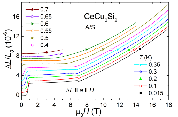
FIG. 2. Length change \Delta L/L_0 normalized to L_0 versus applied magnetic field H \parallel \Delta L \parallel a between zero and 17.9 T is shown for temperatures in the range 0.015–0.7 K. We observe clear steps at the SC transition at 1 T and around 7 T separating phase A from B for lowest temperatures. The anomaly at 1 T shifts to lower fields with increasing T , whereas the step between phase A and B is clearly visible to 0.3 K and gets less pronounced at higher temperature.
