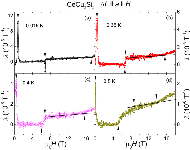
FIG. 3. The magnetostriction coefficient \lambda(H) is shown for four selected temperatures: (a) 0.015 K, (b) 0.35 K, (c) 0.4 K, and (d) 0.5 K illustrating how signatures at the phase transitions (marked with arrows) change with increasing temperature. Please see text for details.
