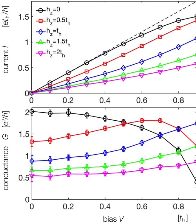
FIG. 10. (Top panel) The current-bias characteristics with different strengths of magnetic field h_z . The dashed black line indicates the perfect conductance with I/V = 2e^2/h . The current is plotted in units of e t_h / h . (Bottom panel) The corresponding plot of the nonlinear differential conductance G = dI/dV against the bias potential V for different magnetic fields h_z . System size is L = 100 for each lead and we use j = 0.35 for which the Kondo temperature is obtained as T_K = 0.4414 t_h from the magnetic susceptibility \chi = 1/(4T_K) .
