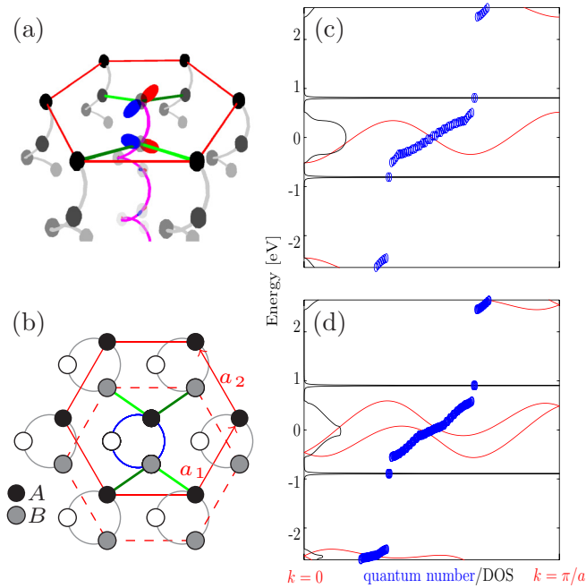
FIG. 1. (a) Schematic view of c -axis surface of the trigonal tellurium lattice formed by van der Waals bonded threefold helices. A red hexagon connects the six surface atoms, highlighted by darker shading, surrounding a central helix in purple. Orbitals represent the local amplitude and phase for the gapped bound-state wave function of a single helix that disperses into a surface band upon coupling with nearest neighbors via light and dark green interhelix bonds. The arXiv version of this paper contains a 3D interactive image when viewed with Adobe Acrobat. (b) Plan view, showing three atoms in the surface unit cell. The solid (dashed) hexagon highlights surface (subsurface) sites denoted as type A ( B ) on nearest-neighbor helices. The contribution from the third site (open circle) in the unit cell is diminished by negligible wave-function amplitude. (c), (d) Energy spectrum for a single one-dimensional helical lattice of tellurium atoms, (c) without and (d) with on-site spin-orbit coupling. Bloch bands in red, discrete spectrum of 50-site finite lattice in blue, and local density of states at the endpoint of a semi-infinite lattice in black. The wave-function orbital components of the gapped bound state in (c) at \approx |V_{\pi}^{(1)}| = 0.8 eV is superimposed on the central helix in (a).
