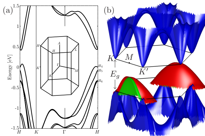
FIG. 2. Electronic band structure of tellurium using a full p_{x,y,z} -orbital tight-binding basis including on-site spin-orbit interaction. (a) shows bulk bands, and (b) shows the projection of a slab spectrum onto the two-dimensional c -axis surface Brillouin zone. Blue surfaces indicate valence and conduction bands delocalized in the bulk; red and green surfaces penetrating the gap highlight the two spin-split bands confined to a single surface.
