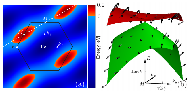
FIG. 3. (a) Analytic model of surface state dispersion, Eq. (1), with matrix elements calculated from the bound state of a single helix without spin-orbit interaction; see Fig. 1(a). Red indicates states above the valence-band maximum, penetrating into the bulk gap. (b) shows anisotropic spin-orbit splitting close to the M -point degeneracy. Colors here correspond to assignments in Fig. 2(b). The directions and lengths of the arrows indicate the orientations of the spin eigenstates, and the strengths of the spin-orbit field, respectively.
