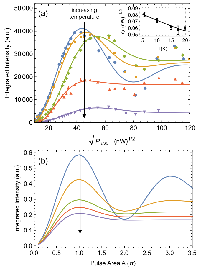
FIG. 3. (a) Rabi oscillations with increasing pulse power recorded for temperatures of T = 5.6, 10, 15, 17.5, 20 \text{ K} , ordered as indicated. The fits in (a) are to a pure-dephasing approximation to the phonon coupling theory. The variation of the oscillation period with temperature, shown by the plot markers in the inset, allows us to extract exciton-phonon coupling parameters, which lead to the solid curve in the inset. At higher temperatures, the maximum of the emitted intensity drops, and the \pi pulse shifts towards more intense excitation power. (b) The result of a full phonon coupling model.
