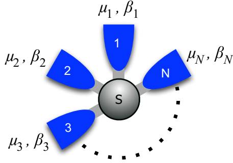
FIG. 1. An open system (S) connected with multiple reservoirs with different inverse temperatures \beta_a and chemical potentials \mu_a for a = 1, \dots, N .
