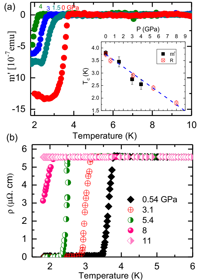
FIG. 5. Temperature dependence of magnetic moment at different values of applied pressure. The inset shows the P - T phase diagram which illustrates the decrease of T_c with the applied pressure. (b) In-plane electrical resistivity of BaPd 2 As 2 versus temperature showing the SC transition for different values of the applied pressure.
