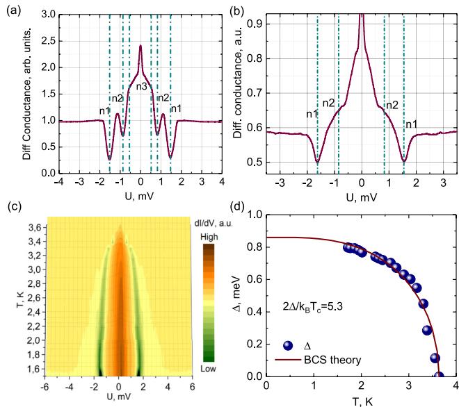
FIG. 4. (a) Dynamic conductance spectrum measured at T = 1.63 K for BaPd 2 As 2 single crystal with local critical temperature T_c = 3.75 K and for SnS Andreev contact with three Andreev reflections. (b) Dynamic conductance spectrum with two Andreev reflections at T = 1.63 K. Vertical green lines in panels (a) and (b) depict the dip positions. (c) Temperature evolution of conductance from the latter junction. (d) Temperature dependence of the obtained superconducting gap. Solid line shows a BCS-like curve for \delta .
