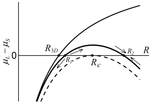
FIG. 1. Oversaturation \mu_L - \mu_S after the nucleation of a crystal of size R , Eq. (14). If the initial oversaturation (\Delta\rho_{SL}/\rho_S\rho_L)\Delta P_L is positive and the volume is infinite then the crystal grows to an infinite size (upper, thin solid curve). Accounting for the finite total volume V shifts the critical radius R_{3D} of the homogeneous 3D nucleation to a larger value R_1 and sets the maximum size of the crystal R_2 (thick solid curve). Decreasing the initial oversaturation brings R_1 and R_2 closer together until they coincide at the critical radius R = R_c(V) , which is the smallest possible stable size of the solid seed (lowest, dashed curve). See text for more details.
