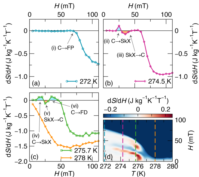
FIG. 4. (a)–(c) shows dS/dH vs H at four representative temperatures. Field-driven phase transitions are easily found: First-order transitions show up as peaks (ii–vi) in this thermodynamic capacity, whereas continuous phase transitions show up as changes in the slope (i). Integration of the peaks gives entropies of transitions and latent heats as shown in Table I. (d) gives a reproduction of the heat map of dS/dH vs T and H as shown in Fig. 3(b) with the slices shown in (a)–(c) overlaid as dashed colored vertical lines. Refer to the caption of Fig. 3 for the definitions of the phase abbreviations.
