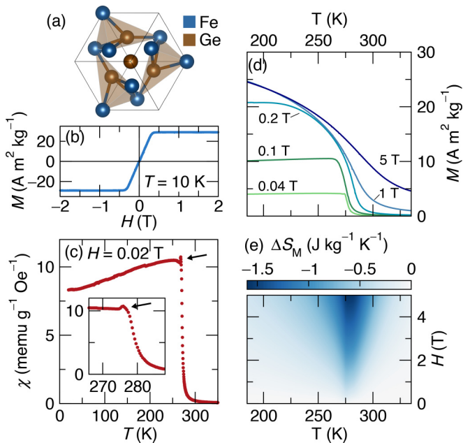
FIG. 1. (a) Crystal structure of cubic B20 FeGe (space-group P2_13 ), shown along the (111) axis. (b) Magnetization as a function of field collected at 10 K is very sharp, saturates at low fields, and shows no hysteresis. (c) Magnetization as a function of temperature collected under applied field H = 20 mT shows an anomaly near T_C . (d) M(T) collected under different applied fields. This is a subset of the dataset (18 total fields) used to calculate the course-grained map of \Delta S_M(H, T) shown in (e).
