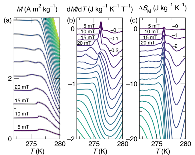
FIG. 2. The process for obtaining high-resolution magnetoentropic information using Eq. (1). (a) dc M(T) data taken at many closely spaced fields (24 fields between 5 and 120 mT) (b) Temperature derivatives of magnetization dM/dT = dS/dH are calculated directly using Tikhonov regularization. For visual clarity, the curves are each offset by 0.1 J \text{kg}^{-1} \text{K}^{-1} \text{T}^{-1} . The antiderivatives of the calculated derivatives are shown as colored lines in (a) and match the raw data (gray crosses) very well. (c) Integrals of the dM/dT curves with respect to the field give the isothermal magnetic entropy change at each temperature and applied field. The curves are each offset by 1 J \text{kg}^{-1} \text{K}^{-1} .
