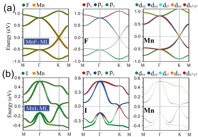
FIG. 4. Energy and \mathbf{k} contribution of atom-resolved (left panel), halogen- p -resolved (middle panel), and Mn- d -resolved (right panel) to the majority-spin bands for (a) MnF 3 and (b) MnI 3 using the HSE06 functional. The color intensity denotes the amplitude of the atom- and/or orbital-resolved character.
