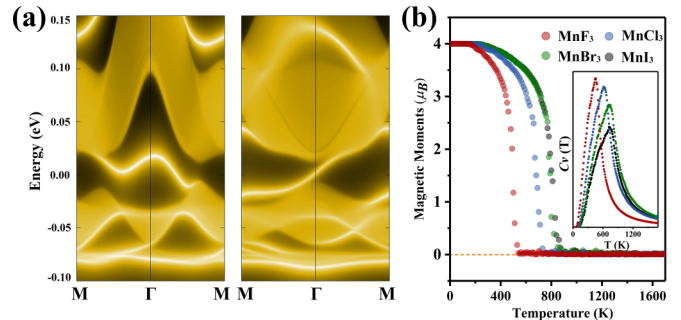
FIG. 5. (a) Band structure of the zigzag (left) and the armchair (right) edges of the MnBr 3 ribbon, with the edge states connecting the 2D valence and conduction bands. (b) Temperature variation of the Mn 3+ magnetic moment for the 2D MnX 3 . (Inset) Temperature variation of the heat capacity.
