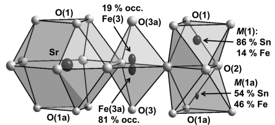
FIG. 2. Section of the crystal structure of \text{SrSn}_2\text{Fe}_4\text{O}_{11} . Sr is coordinated by twelve oxygen atoms that define a nearly ideal anticuboctahedron. Face-sharing octahedral sites have mixed occupation by Sn/Fe atoms with different ratios ( M(1) by 86% Sn, M(1a) by 54% Sn). Face-sharing tetrahedra are occupied to a different extent: Fe(3) to 19%, Fe(3a) to 81%, which corresponds to a shift of the Fe(3a) atoms by about 0.2 \text{ \AA} off the ideal center position along [001] in the trigonal bipyramidal void. Atoms are depicted with displacement ellipsoids with 90% probability.
