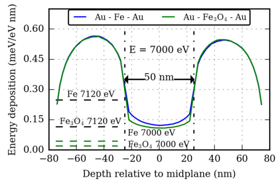
FIG. 5. Linear energy deposition in layered Au-Fe-Au and Au-Fe 3 O 4 -Au targets of 150 nm total thickness stimulated by 7 keV photons (solid curves). Dashed lines on the left indicate energy deposition in bulk Fe 3 O 4 and Fe at photon energies of 7.12 keV (above the Fe K-edge) and 7 keV (below the edge). The multilayer configuration sufficiently enhances energy deposition so as to partially compensate for the difference between pre- and above-edge x-ray photoelectric cross sections. The benefit is particularly pronounced in Fe 3 O 4 due to its much lower density and photoelectric cross-section.
