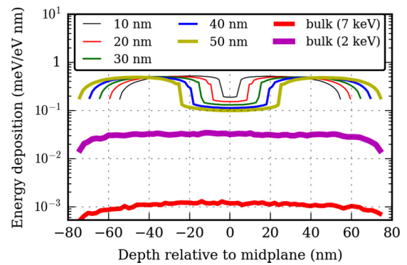
FIG. 3. Linear energy deposition due to 7 keV photons incident on an Au-C-Au target displayed for several thicknesses of the central C layer and a fixed outer cladding thickness of 50 nm, compared to the linear energy deposition created by 7 and 2 keV photons incident on bulk C. The large, expected decrease in direct absorption of the higher-energy x rays by the unclad samples is more than compensated by the nonlocal heating from electron transport between the Au and the interior material for the Au-C-Au target.
