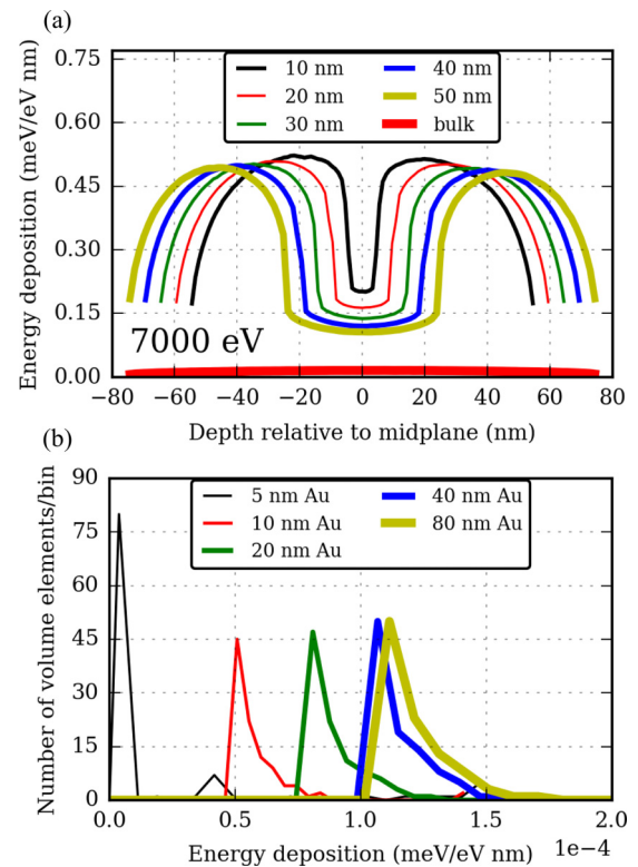
FIG. 4. (a) Linear energy deposition density generated by 7 keV photons incident on an Au-Fe 3 O 4 -Au target, displayed for several thicknesses of the central Fe 3 O 4 layer and a fixed Au cladding thickness of 50 nm. (b) Histograms of energy deposition density in volume elements of the Fe 3 O 4 inclusions in Au-Fe 3 O 4 -Au targets, displayed for several thicknesses of the Au cladding and a fixed Fe 3 O 4 layer thickness of 50 nm.
